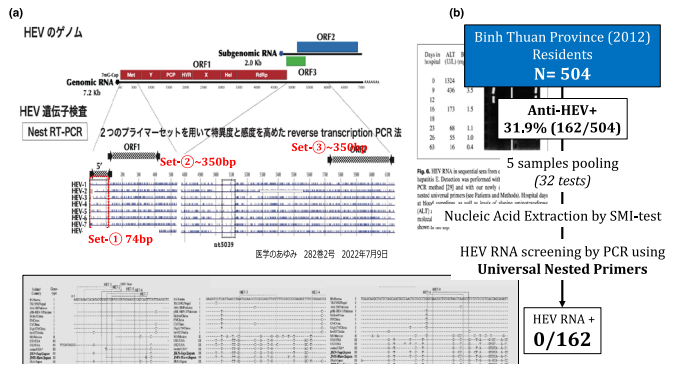
Figure 4: (a) Sketch diagram of universal primer sets used for HEV RNA amplification and (b) its result
