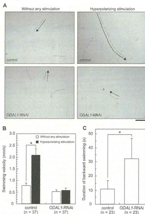
FIG 3 Phenotypes of ODAL1 -RNAi cells. Swimming behaviors of control cells and ODAL1 -RNAi cells (2 days after the induction of gene silencing) were observed under certain conditions. Observation and recording were performed as indicated in Materials and Methods. (A) Swimming paths of live paramécia for 1 s without any stimulation and in response to hyperpolarizing stimulation by the addition of \text{CaCl}_2 to attain a \text{Ca}^{2+} concentration of 2 mM. The frame capture rate was 15 frames per s. The arrows indicate the swimming directions. Bar, 0.5 mm. (B) Forward swimming velocity in control cells and ODAL1 -RNAi cells. In the case of the control, the difference between the swimming velocities under standard conditions and under conditions of hyperpolarizing stimulation was significant (*, P < 0.01 by t test). In the case of ODAL1 -RNAi cells, the difference was not significant. (C) Duration of backward swimming in control and ODAL1 -RNAi cells. Backward swimming was induced by depolarizing stimulation by the addition of KCl to attain a \text{K}^+ concentration of 50 mM. The difference between the durations of backward swimming in control and ODAL1 -RNAi cells was significant (*, P < 0.001 by t test). Boxes and bars indicate means \pm standard deviations (SD), respectively. The number of measurements is indicated in each panel (B and C).
