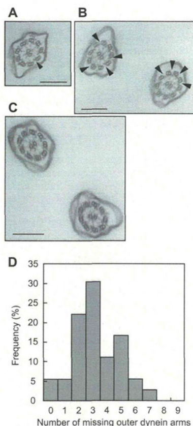
FIG 8 Transmission electron micrographs of cross sections of ODAL1 -RNAi cilia. Typical cross-sectional images of cilia from ODAL1 -RNAi (2 days after the induction of gene silencing) (A and B) and ND7 -RNAi (C) cells were observed by using a transmission electron microscope. The arrowheads indicate the positions of the missing outer dynein arms on the outer doublet microtubules. Bars, 200 nm. (D) Histogram of missing outer dynein arms in ODAL1 -RNAi axonemes. The abscissa indicates how many outer dynein arms were missing ( n = 36 ).
