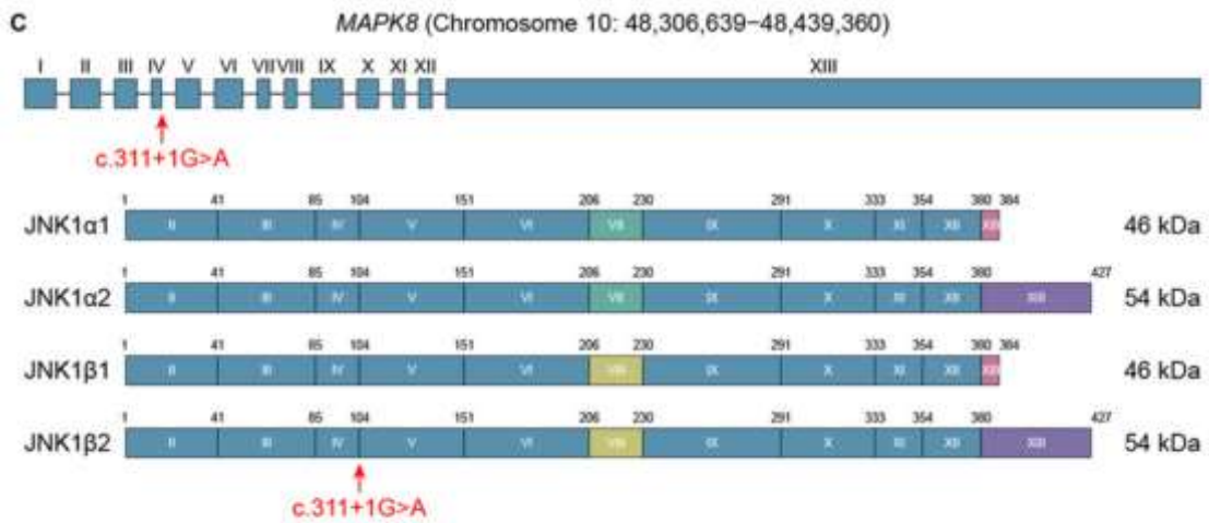
Fig. 1. Identification of a heterozygous MAPK8 mutation in a kindred with AD CMC and CTD.
