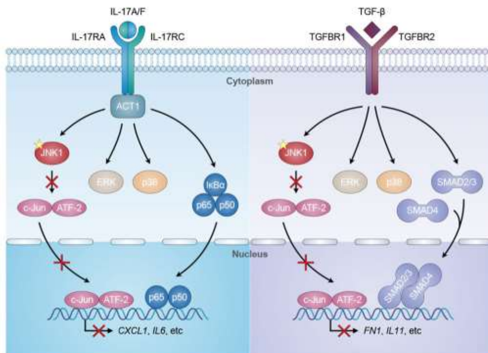
Fig. 6. JNK1-dependent IL-17 and TGF- \beta signaling.
