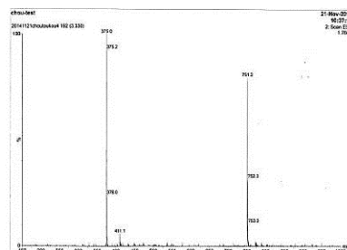
単離化合物の LC/MS (Waters) (negative mode)
