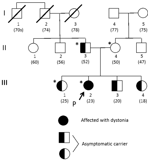
図2. GCH1-DYT5, c.325T>C (p.Y109H)
