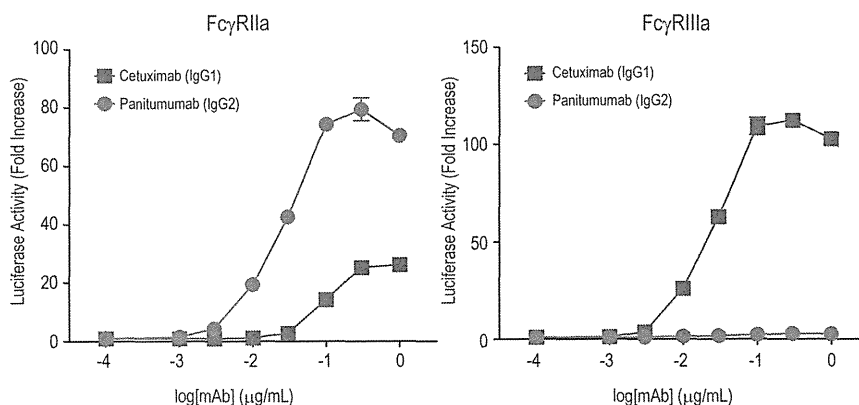
Figure 3. Activation of Jurkat/Fc \gamma R/NFAT-Luc cells by EGFR-bound cetuximab and panitumumab. A431 and Jurkat/Fc \gamma R/NFAT-Luc cells were co-cultured in the presence of serially diluted cetuximab (IgG1 subclass) or panitumumab (IgG2 subclass). The luciferase activity (i.e., the fold increase compared to the control sample without mAbs) is represented on the graphs. The assays were performed in triplicate, and the data are the mean \pm SEM. Panitumumab activated Jurkat/Fc \gamma RIIa/NFAT-Luc cells more strongly than cetuximab ( p <0.0001, Graphpad Prism Software). doi:10.1371/journal.pone.0095787.g003
