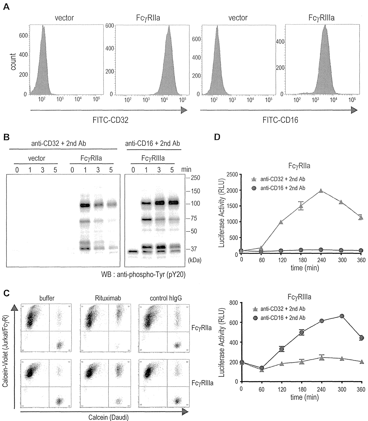
Figure 1. Establishment of the Fc \gamma R-expressing reporter cell lines. (A) The cell surface expressions of Fc \gamma R in Jurkat/Fc \gamma R cells were analyzed by flow cytometric analysis. (B) The crosslinking of Fc \gamma R by anti-Fc \gamma R monoclonal antibodies induced the tyrosine-phosphorylated proteins in Jurkat/Fc \gamma R cells. (C) Bridging between calcein-labeled Daudi and calcein-violet-labeled Jurkat/Fc \gamma R cells via rituximab was analyzed by flow cytometry. (D) The crosslinking of Fc \gamma R by anti-Fc \gamma R monoclonal antibodies induced the luciferase activities in Jurkat/Fc \gamma R/NFAT-Luc cells. The assays were performed in triplicate, and the data are the mean \pm SEM. doi:10.1371/journal.pone.0095787.g001
