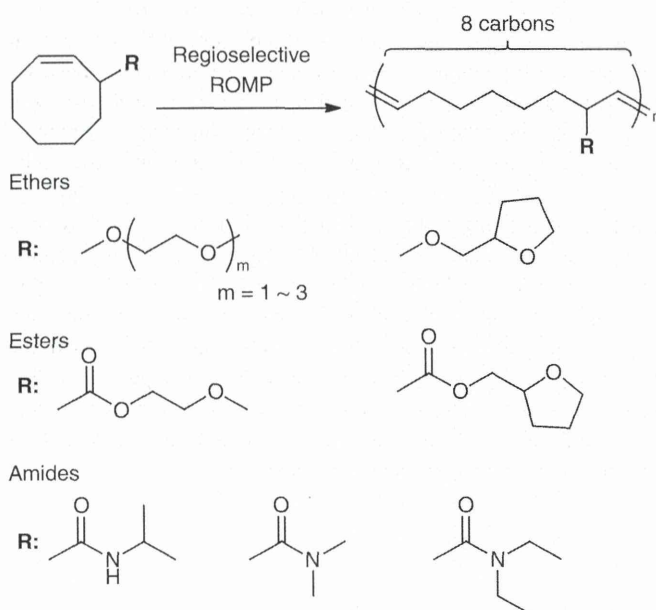
Figure 5 Synthesis of polymers having precisely placed side-chain branches by regio- and stereo-selective ROMP of allyl-substituted cis -cyclooctenes.
