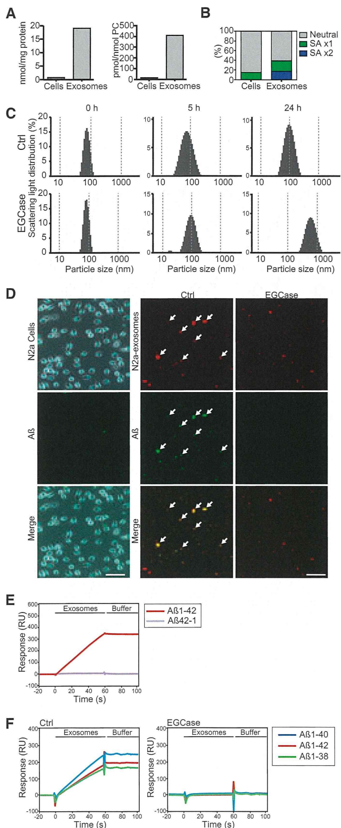
FIGURE 5. Exosomal GSLs are responsible for A \beta binding on the vesicles. Exosomal and cellular glycomics of GSLs were surveyed by mass spectrometry. A , total amounts of GSL-glycans in exosomes and their originating cells were determined by standardization with protein or phosphatidylcholine (PC) content. B , GSLs other than GM2 detected in exosomes or cells were classified according to the number of sialic acid moieties. C , particle size of exosomes (untreated or treated with EGCase) was determined by dynamic
