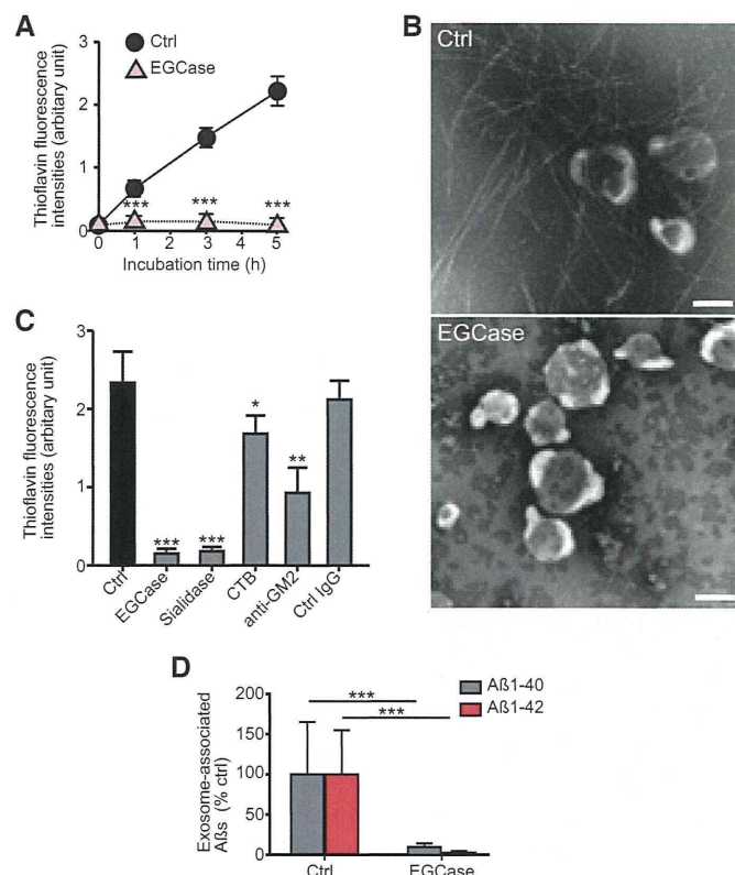
FIGURE 6. Exosomal GSLs are involved in A \beta assembly. A , thioflavin fluorescence intensities were measured in mixtures of exosomes (untreated as Ctrl or treated with EGCase) incubated with 15 \mu M A \beta_{1-42} . Data are presented as the mean \pm S.D.; ***, p < 0.001 ( n = 4 ). B , representative electron microscopic images of exosomes incubated for 5 h with 15 \mu M A \beta_{1-42} are shown. Scale bar, 100 nm. C , the exosomes (untreated as Ctrl or treated with EGCase or sialidase) were incubated for 5 h with 15 \mu M A \beta_{1-42} . The untreated exosomes were reacted with A \beta in the presence of cholera toxin B subunit (CTB) or anti-GM2 antibody. Fluorescence intensities of thioflavin-T were then measured. Values in each column are the mean \pm S.D. of five values. *, p < 0.05 ; **, p < 0.01 ; ***, p < 0.001 . D , biotinylated exosomes (untreated as Ctrl or treated with EGCase) stereotactically injected into the hippocampus of APP mice (4 months) were isolated at 3 h after the injection, and the levels of exosome-associated A \beta were quantified by ELISA. Values are the mean \pm S.D., ***, p < 0.001 ( n = 4 ).
