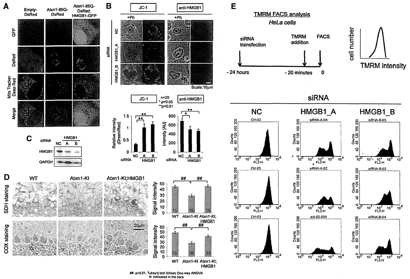
Figure 3. HMGB1 restores mitochondrial functions.
