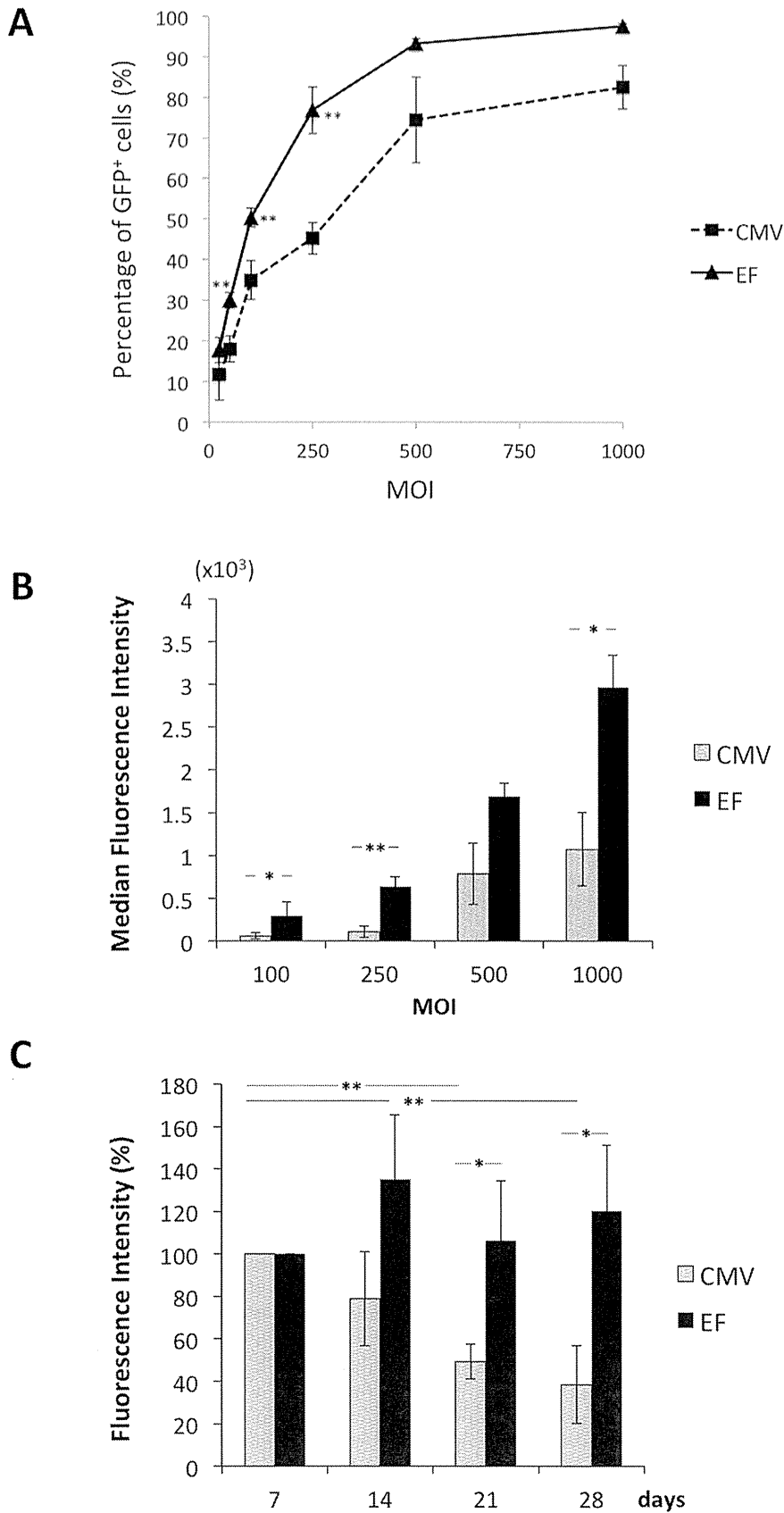
Figure 1. The efficiency of CMV or EF-1 \alpha promoter in hADMPCs. Lentiviral vectors encoding EGFP under the control of CMV or EF-1 \alpha promoter were transduced with hADMPCs at m.o.i. of 25, 50, 100, 250, 500, and 1000, and the cells were analyzed by flow cytometry. (A) The percentage of EGFP-positive hADMPCs transduced with CSII-CMV-EGFP (CMV) or CSII-EF-EGFP (EF). (B) (C) The median fluorescence intensities of the
