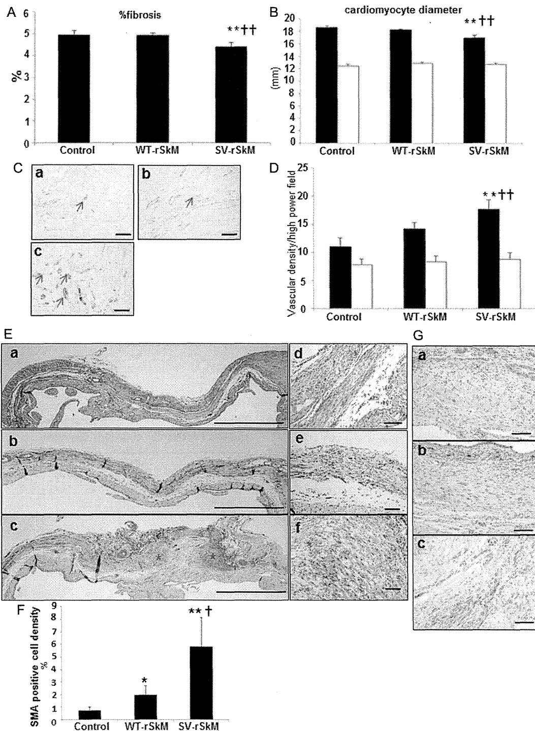
Figure 3 Histological evaluations of LV remodelling. (A) Percentage fibrosis. (B) Cardiomyocyte diameter. **P < 0.01 vs. Control group. ^{\dagger\dagger}P < 0.01 vs. WT-rSkM group. Filled bars, border area; open bars, remote area. Immunohistochemical staining. (C) A section of the infarcted border zone stained with an antibody against von Willebrand factor: (a) control; (b) WT-rSkM; and (c) SV-rSkM ( \times 200 magnification, scale bars represent 100 \mu\text{m} ). Newly formed vessel is stained brown. (D) Quantitative estimation of vascular density. **P < 0.01 vs. Control group. ^{\dagger\dagger}P < 0.01 vs. WT-rSkM group. Filled bars, border area; open bars, remote area. (E) The distribution of SMA-positive cells: (a) control; (b) WT-rSkM; (c) SV-rSkM (a–c, \times 20 magnification, scale bars represent 1000 \mu\text{m} ; e and f, \times 200 magnification, scale bars represent 100 \mu\text{m} ). Red asterisks denote SMA-positive cells. (F) Quantitative estimation of the SMA-positive cell density. *P < 0.05 , **P < 0.01 vs. Control group. ^{\dagger}P < 0.05 vs. WT-rSkM group. (G) The distribution of SM-MHC type 2-positive cells: (a) control; (b) WT-rSkM; and (c) SV-rSkM (a–c, \times 200 magnification, scale bars represent 100 \mu\text{m} ).
