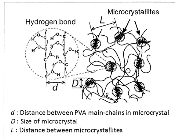
Figure 13. Network structure of PVA hydrogels crosslinked by microcrystallites. 38
