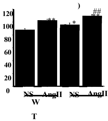
Figure 12. Urinary TP/Cr
