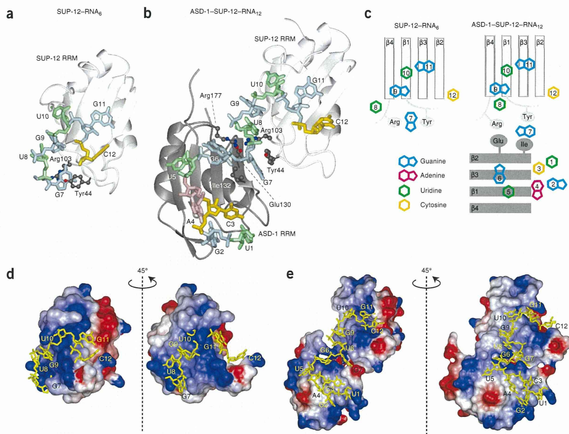
Figure 2 Solution structures of SUP-12-RNA 6 and ASD-1-SUP-12-RNA 12 complexes. (a,b) Ribbon representations of the SUP-12-RNA 6 complex (a) and the ASD-1-SUP-12-RNA 12 complex (b) . SUP-12 RRM and ASD-1 RRM are colored white and gray, respectively. The G, A, U and C nucleotides are shown in light blue, pink, light green and yellow, respectively. The side chains in the RRM domains involved in the G7-base recognition are represented as follows: black, carbon; red, oxygen; blue, nitrogen. (c) Schematic diagrams of the SUP-12-RNA 6 complex (left) and the ASD-1-SUP-12-RNA 12 complex (right). (d,e) Electrostatic-potential surfaces of the RRM domains in the SUP-12-RNA 6 complex (d) and the ASD-1-SUP-12-RNA 12 complex (e) . Red and blue indicate negative and positive charges, respectively. The RNA molecule is colored yellow.
