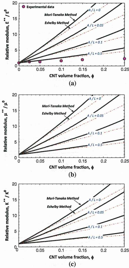
Fig. 3 Effects of CNT volume fraction on the effective elastic moduli of CNT–polystyrene composites [35] (cf. [1, 34]). a Variations of effective Young’s modulus, E^{**} . b Variations of effective shear modulus, \mu^{**} . c Variations of effective bulk modulus, K^{**} . E^1 = 1.0 TPa, \nu^1 = 0.3 , E^0 = 1.9 GPa, \nu^0 = 0.3
