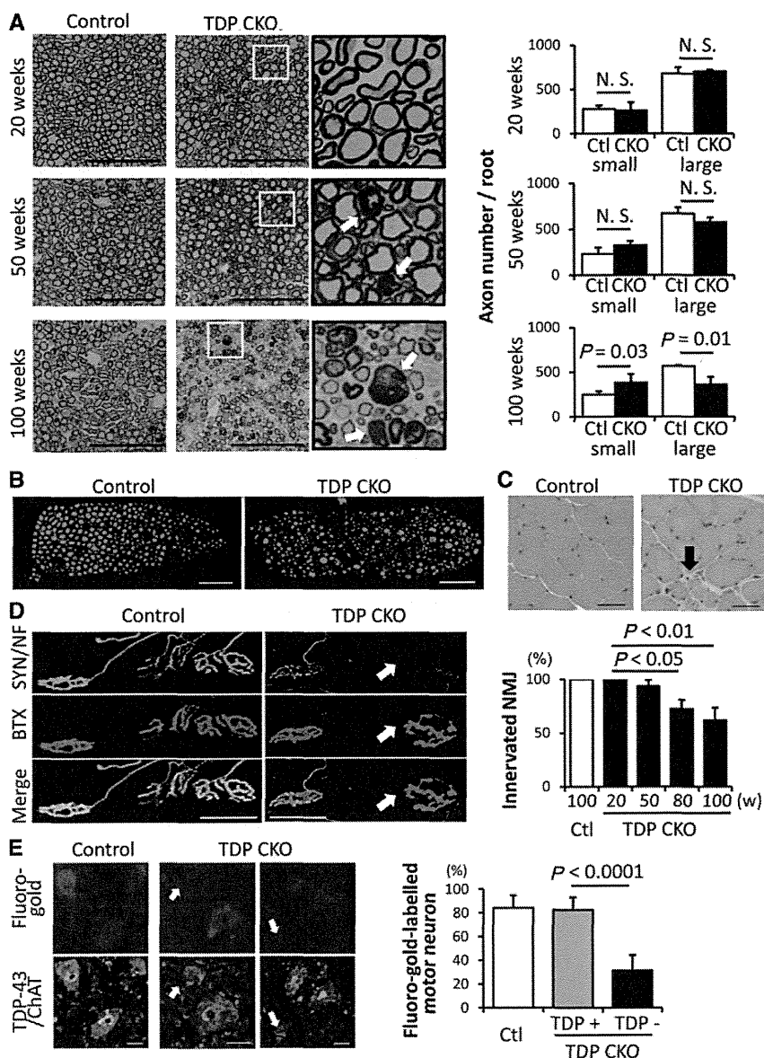
Figure 3 Analysis of motor axons, neuromuscular junctions, and skeletal muscles. (A) Toluidine blue staining images and the number of small myelinated fibres (<5 µm) and large myelinated fibres (>5 µm) in the L5 ventral root from 20, 50 and 100-week-old control and TDP CKO mice (n = 6 axons of each). The enlarged image of the yellow-framed area is also shown. Arrows indicate axonal degenerations. Scale bars = 100 µm. Error bars indicate SD. (B) Immunofluorescent staining of the L4 ventral root in 100-week-old mice with an anti-ChAT antibody. (C) Haematoxylin and eosin staining of gastrocnemius muscles of 100-week-old mice. Axial sections from TDP CKO mice exhibited grouped atrophy (arrow), whereas the control littermates showed no such phenomenon. (D) Immunofluorescent staining [synaptophysin (SYN) and phospho-neurofilament (NF), green; bungarotoxin (BTX), red] of neuromuscular junctions (NMJ) in 100-week-old mice and a time course analysis of neuromuscular junctions in TDP CKO mice. Denervated neuromuscular junctions (arrow) are indicated by the lack of synaptophysin and phospho-neurofilament staining. Scale bars = 50 µm. Error bars indicate SD (n = 3). (E) FluoroGold labelling (blue) and immunofluorescence staining (TDP-43, green; ChAT, red) of lumbar motor neurons. Retrograde FluoroGold labelling was significantly attenuated in TDP-43-lacking motor neurons but not in TDP-43-positive neurons in 100-week-old TDP CKO mice (arrows). Scale bars = 20 µm. Error bars indicate SD (n = 10).
