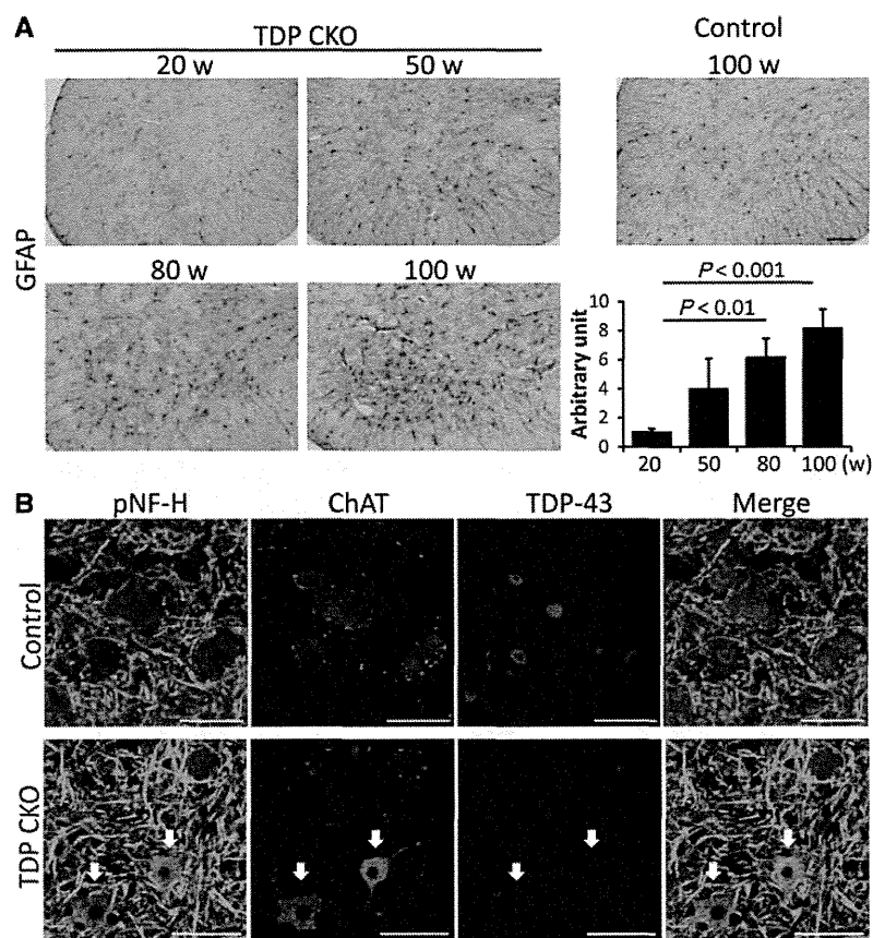
Figure 5 Astroglisis and neuronal accumulation of phosphorylated neurofilament. (A) Immunohistochemistry against GFAP in the ventral horn and a time course analysis of astroglisis. Error bars indicate SD ( n = 3 for each age). (B) Immunofluorescent staining against pNF-H (green), ChAT (red) and TDP-43 (blue). pNF-H was accumulated in the cell bodies of TDP-43-lacking motor neurons of TDP CKO mice (arrows). Scale bars: A = 100 \mu m; B = 50 \mu m.
