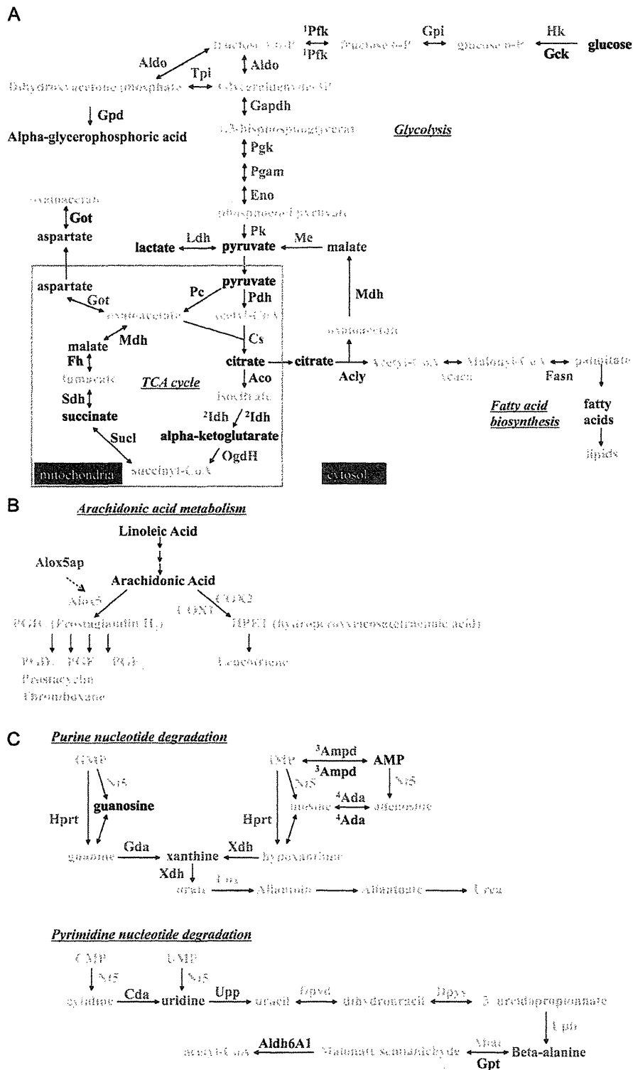
Fig. 3. Schematic representations of the most relevant metabolic and transcriptional differences in pancreatic tissues between PDAC and normal rats. Red, higher concentration in PDAC rats. Blue, lower concentration in PDAC rats. Black, not changed. Gray, not determined or unclear. 1 Pfkm was increased, whereas Pfk was decreased. 2 Idh3a was increased, whereas Idh2, Idh3B and Idh3g were decreased. 3 Ampd3 was increased, whereas Ampd2 was decreased. 4 Ada, Adarb1 and Adarb2 were increased, whereas Adar was decreased.
