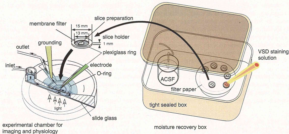
Fig. 2. An illustration of the experimental chamber system. The illustration on the left shows the experimental chamber, holding a slice preparation held on top of a membrane filter supported by the plexiglass ring (the slice holder ring). The physiological solution is fed to the chamber from an inlet and run under the membrane filter; then it flows over the slice and is sucked up by an outlet tube. An electrical ground was installed near the outlet port. The slice can be accessed by electrode and can be observed with transmitted light and epi-fluorescence. The slice holder rings, along with a slice, are placed on filter paper covering on a container filled with physiological solution, which is kept in the tight sealed box filled with moist air with \text{CO}_2/\text{O}_2 gas bubbled into the solution. When staining the slice, an aliquot of staining solution ( 100 \mu\text{l} ) is applied to the slice holder, which should be washed out after the proper staining duration.
