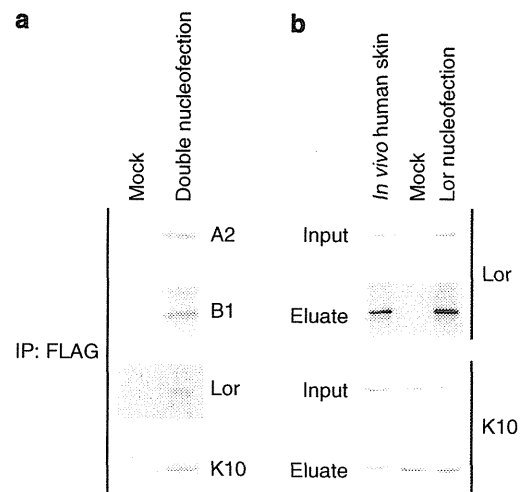
Figure 4. Association of the profilaggrin N -terminus with loricrin and keratin 10 (K10). (a) HaCaT cell were doubly nucleofected with pFLAG467proF and pcDNA3.1/V5-His-loricrin. The cells were lysed and processed for FLAG immunoprecipitation (IP) followed by A2, B1, loricrin (Lor), and K10 immunoblotting ( n = 4 ). The immunoprecipitates of FLAG contained loricrin and K10. (b) Glutathione S -transferase (GST) pull-down assays. GST-tagged profilaggrin N -terminal domain (PND) was immobilized on glutathione beads and probed for an interaction with Lor and K10. Binding of GST-tagged PND to loricrin or K10 was determined by immunoblot analyses ( n = 4 ).
