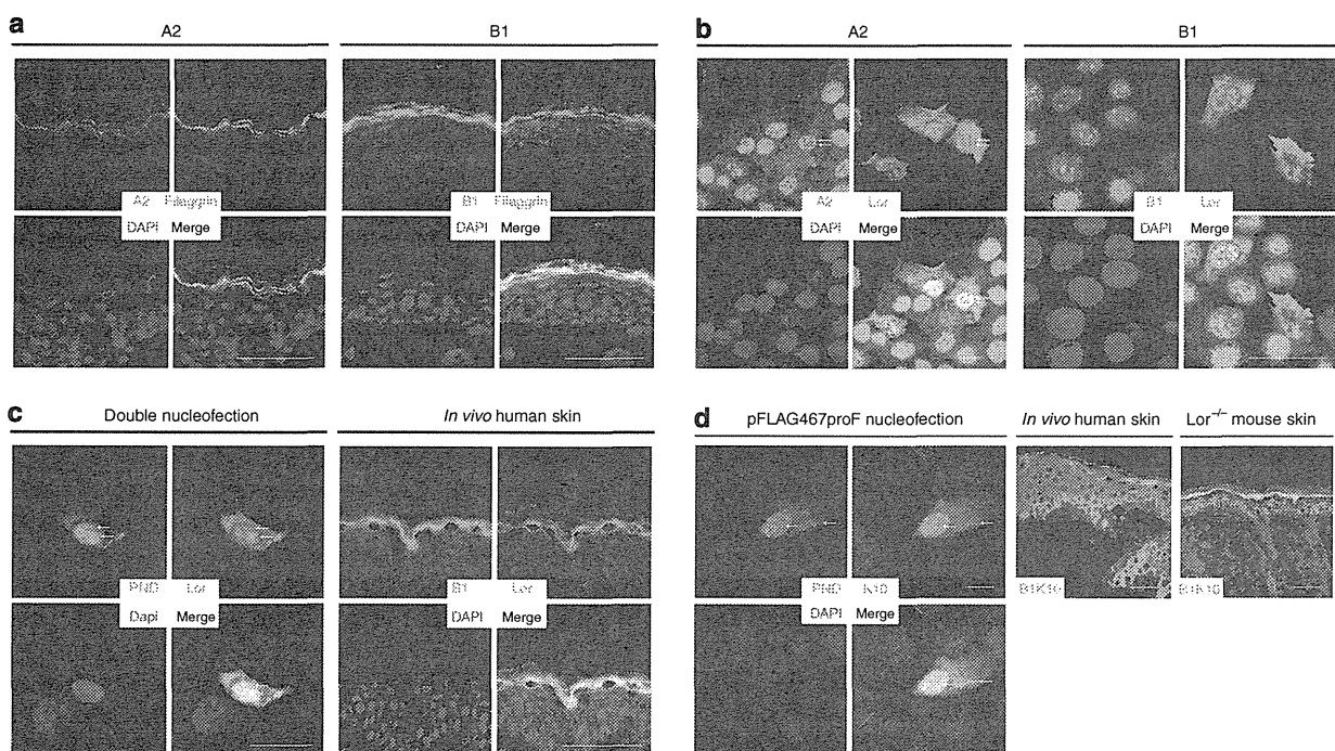
Figure 1. Expression of the A and B domains of profilaggrin N-terminal domain (PND) in human adult epidermis and HaCaT cells and colocalization with loricrin. (a) We prepared cryosections from optimal cutting temperature (OCT) compound-embedded normal human skin. We conducted double immunostaining with filaggrin mAb AKH1 and A2 or B1 antibody. A2 and B1 immunostained cytoplasm of granular layers and also showed some reaction with the lower stratum corneum. DAPI, 4,6-diamidino-2-phenylindole. Bars = 80 \mu m. (b) Distribution of PND in HaCaT cells nucleofected by pcDNA3.1/V5-His-lovicrin. Nucleofected HaCaT cells were fixed at 48 hours after transfection, and the cells were stained with anti-V5 antibody and either A2 or B1 antibody. Nucleofected loricrin distributed diffusely in the cytoplasm and in the nuclei. PND also distributed in the nuclei abundantly and the cytoplasm in HaCaT cells. A substantial portion of nucleofected loricrin colocalized with PND (arrows). Bars = 50 \mu m. Interaction of PND and loricrin (Lor). (c) We doubly nucleofected pFLAG467proF and pcDNA3.1/V5-His-lovicrin into HaCaT cells. Cells were fixed at 48 hours after transfection, and the fate of the transfected gene product was examined by double-label immunofluorescence. To visualize the nucleofected gene product, cells were doubly stained with a rabbit polyclonal antibody recognizing the sequence of FLAG tag and a mouse mAb recognizing the sequence of V5 tag. PND distributed in the nuclei and diffusely in the cytoplasm in nucleofected cells. PND and loricrin (Lor) colocalized not only in the cytoplasm but also in the nucleus (arrows). Bar = 25 \mu m. We also doubly stained in vivo human skin with B1 antibody and guinea pig polyclonal anti-lovicrin antibody. PND and Lor colocalized in the cytoplasm of granular cells and the lower cornified cells. Bars = 80 \mu m. (d) We doubly stained HaCaT cells nucleofected with pFLAG467proF with B1 antibody and mouse anti-K10 mAb. PND and keratin 10 (K10) colocalized not only in the nucleus but also in the cytoplasm. Bar = 10 \mu m. We doubly stained in vivo human skin with B1 antibody and mouse anti-K10 mAb. PND and K10 colocalized at granular layer and lower stratum corneum. We doubly stained Lor -/- mouse skin with B1 antibody and mouse anti-K10 mAb. PND and K10 colocalized at granular layer and lower stratum corneum. Bars = 80 \mu m.
