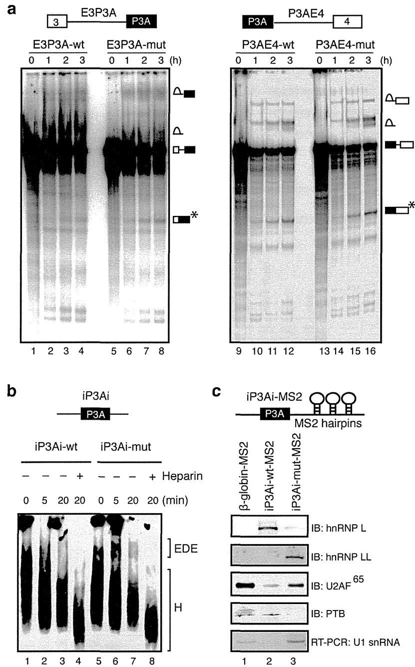
Figure 5 | Skipping of exon P3A is promoted by impairing the formation of exon-defined E (EDE) complex in the wild-type pre-mRNA. (a) Time-course data obtained from in vitro splicing of the ^{32}\text{P} -labeled pre-mRNAs from E3P3A (wt and mut) and P3AE4 (wt and mut) minigenes. The splicing products are shown schematically on the right. The spliced mRNA (asterisk) is increased in E3P3A-mut compared to E3P3A-wt. Although intron lariats are apparently increased in E3P3A-wt, the intron lariat and high molecular weight RNAs are not clearly resolved for E3P3A, and the increase of the intron lariats cannot be precisely estimated. Poor resolution of splicing products of E3P3A compared to P3AE4 is likely due to binding of a splicing repressing PTB. (b) Time-course analysis of early exon-defined spliceosome (EDE complex) that assembles across the P3A exon of ^{32}\text{P} -labeled substrates (iP3Ai-wt and iP3Ai-mut) in the absence of ATP. Native agarose gel electrophoresis resolves the indicated nonspecific complex H (H) and the exon-defined E complex (EDE). (c) Schematic structures of MS2-attached wild-type (wt) and mutant (mut) substrates used for isolation of EDE complex. Immunoblotting (IB) and RT-PCR analyses of purified E complex assembled on indicated substrates. PTB was likely bound to a CUCUCUCU sequence in intron 1 of \beta -globin-MS2 pre-mRNA.
