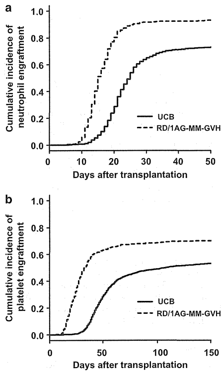
Figure 1. Neutrophil (a) and platelet engraftment (b).
