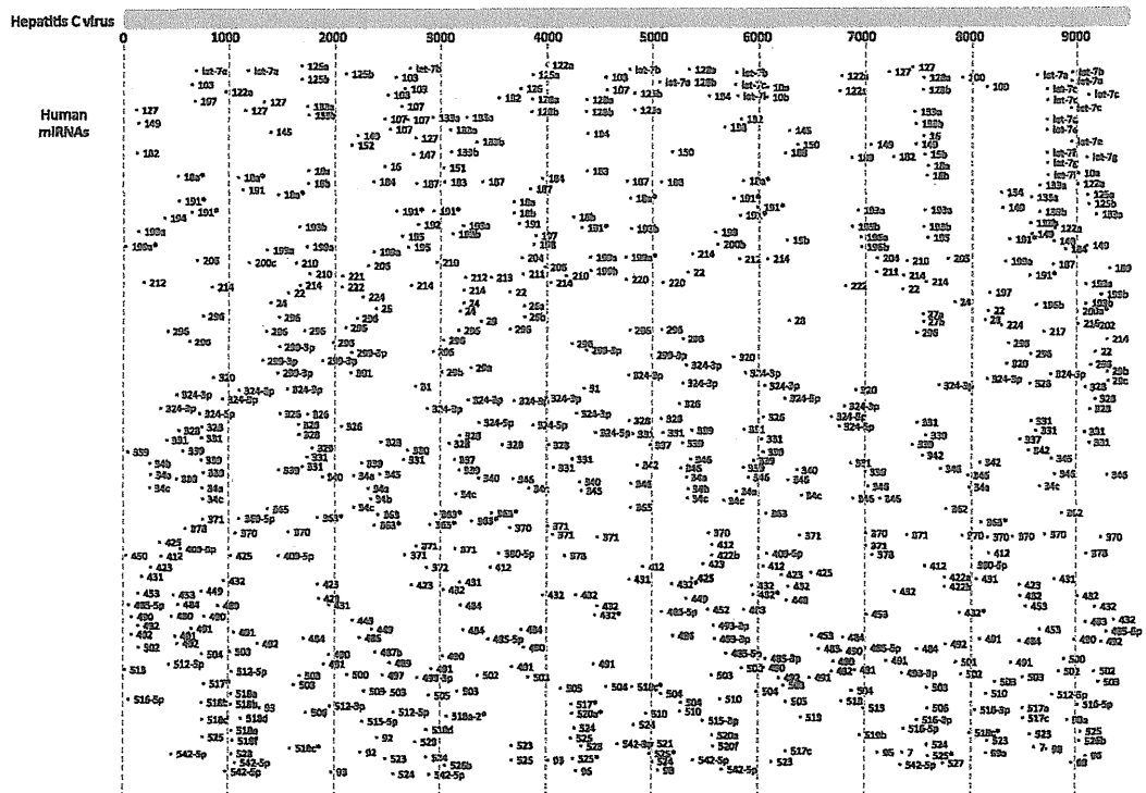
Fig. 7.4 Hypothetical miRNAs target sites on HCV genome
