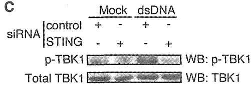
Figure 9. p-TBK1 levels in IPS-1 or STING knockdown cells. (A-C) siRNA for negative control, IPS-1, or STING were transfected into HeLa cells. At 48 h after transfection, cells were stimulated with HBV F1 fragment or salmon sperm DNA for 6 h. Cells were fixed and stained with Mitotracker Red and anti-p-TBK1 antibody (A), or cell lysates were prepared and subjected to SDS-PAGE and western blotting (B and C).
