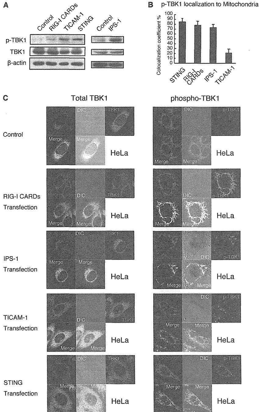
Figure 1. Mitochondrial localization of p-TBK1 in HeLa cells. (A) HeLa cells were transfected with 1.2 μg of empty vector, RIG-I CARDs, TICAM-1, IPS-1, or STING expression vectors in 6-well plate. At 24 h after transfection, cell lysates were prepared and subjected to SDS-PAGE. Proteins were detected by western blotting using anti-TBK1, p-TBK1, and β-actin antibodies. (B and C) HeLa cells were transfected with 0.3 μg of empty vector or RIG-I CARDs, TICAM-1, or STING expression vectors in 24-well plate. At 24 h after transfection, cells were fixed and stained with anti-TBK1 or anti-p-TBK1 antibodies and Mitotracker Red. Colocalization coefficients of p-TBK1 with mitochondria were determined (mean ± sd, n = 3) (C). Unless otherwise indicated, Data are from one representative (n = 3) of at least three independent experiments. doi: 10.1371/journal.pone.0083639.g001
