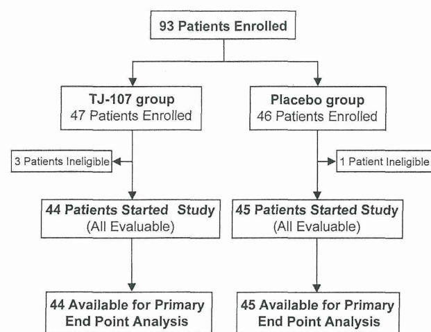
Fig. 1 CONSORT diagram
