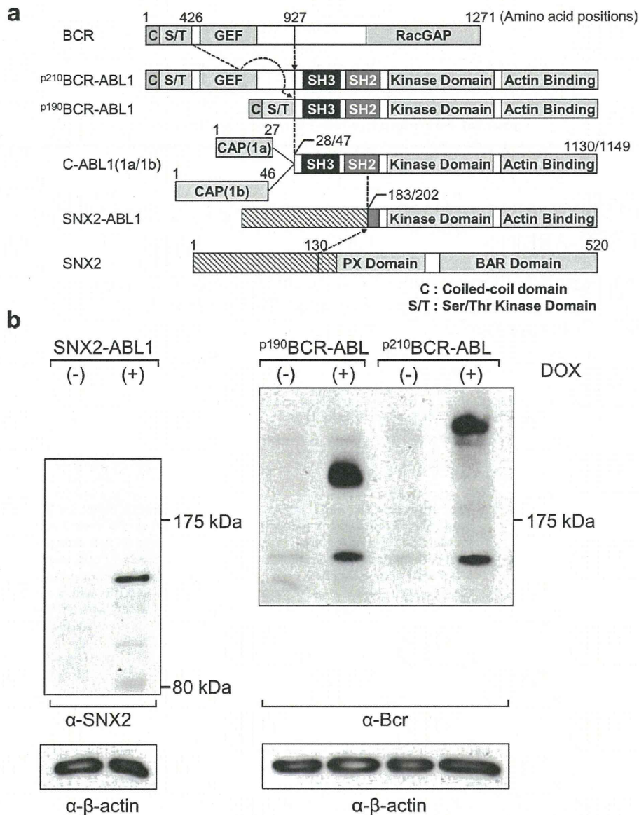
Fig. 1. Structure and expression of SNX2-ABL1 kinase. (a) Structures of SNX2-ABL1, p 190 BCR-ABL1 and p 210 BCR-ABL1 kinases are schematically presented. Amino acid positions of recombination sites are also indicated. (b) Doxycycline-induced protein expressions of SNX2-ABL1 and p 190 /p 210 BCR-ABL1 in Ba/F3 cells were detected by immunoblotting using the indicated antibodies. Molecular mass references (kDa) are indicated. Simultaneously, β-actin was blotted as a loading control.
