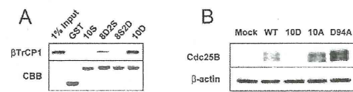
Fig. 7. A peptide encompassing the region between E 82 SS and S 101 PSP is a possible \beta TrCP-binding sequence in Cdc25B. (A) GST-fused Cdc25B-derived peptides consisting of the sequence E 82 SS to S 101 PSP were mixed with crude cell extracts prepared from Myc-tagged \beta TrCP1-transfected Cos7 cells, and this was followed by the recovery of proteins bound to GST-fused peptides. The recovered \beta TrCP1 was detected with anti-Myc antibody. The reaction mixture included 1 \mu M staurosporine to avoid the phosphorylation of Ser residues in the peptides by kinases present in the cell extracts. (B) FLAG-Cdc25B of wild type, 10D (all Ser residues in E 82 SS to S 101 PSP were replaced with Asp), 10A (all Ser residues in E 82 SS to S 101 PSP were replaced with Ala) or D94A were transfected into HeLa cells and their expression was determined by immunoblotting.
