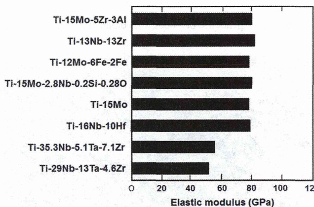
Figure 3. Elastic moduli of \beta -type alloys [4].
