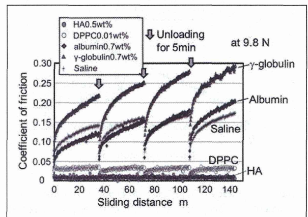
Figure 7. Influence of each synovial constituent on changes in friction of freeze-thawing PVA hydrogel against glass plate. PVA: poly(vinyl alcohol).
