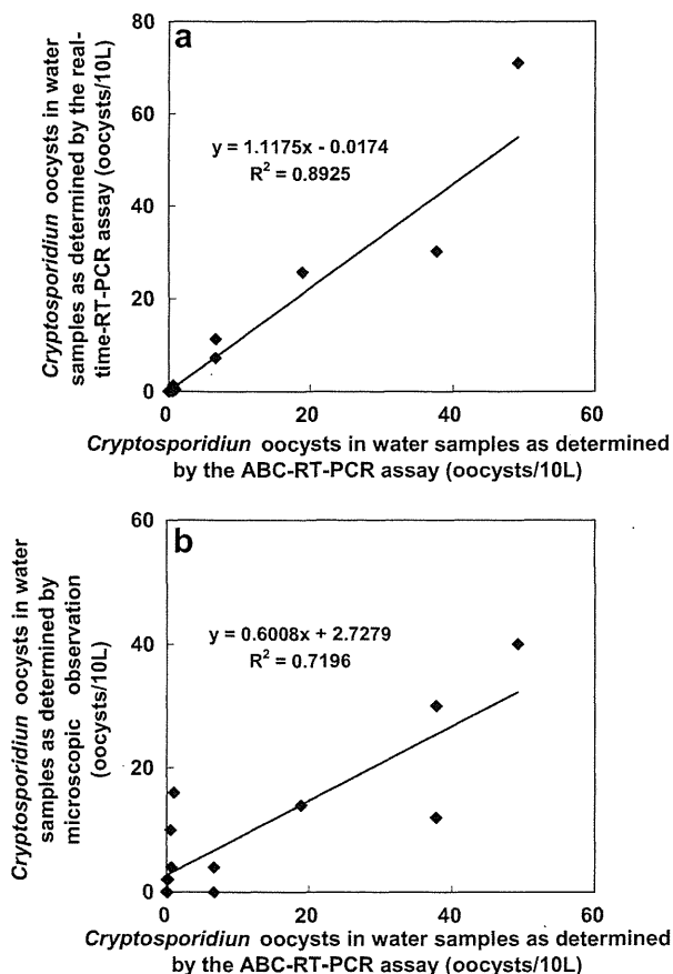
Fig. 4 – Relationship between the number of Cryptosporidium oocysts in water samples as determined by (a) ABC-RT-PCR and real-time RT-PCR (b) ABC-RT-PCR and microscopic observation.
