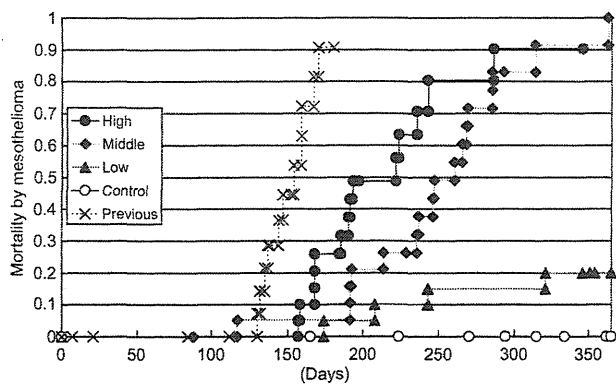
Fig. 1. Dose-dependent induction of mesotheliomas by micrometer-sized multi-wall carbon nanotubes ( \mu m-MWCNT). Mice with lethal mesotheliomas are plotted using the Kaplan–Meier method. High: 300 \mu g/mouse, corresponding to 1 \times 10^8 fibers/mouse; middle: 30 \mu g/mouse, corresponding to 1 \times 10^7 fibers/mouse; low: 3 \mu g/mouse, corresponding to 1 \times 10^6 fibers/mouse; previous: data from a previous study (i.e. 3 mg/mouse, corresponding to 1 \times 10^9 fibers/mouse). No mesothelioma was observed in the vehicle control group.
