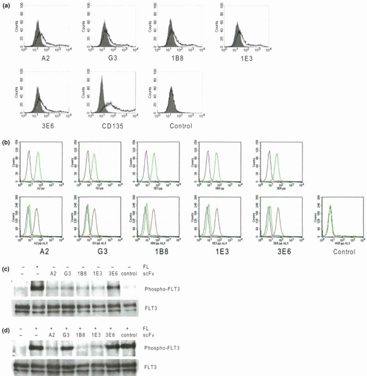
Fig. 1. FMS-related tyrosine kinase 3 (FLT3)-binding assay analyses and effects of isolated Abs on FLT3 phosphorylation. (a) FLT3-binding activity of the scFv form of A2, G3, 1B8, 1E3, and 3E6 Abs were examined using flow cytometry (FCM). CD135 is a polyclonal Ab against FLT3 and was used as a positive control. Open histogram represents the staining of FLT3-transfected 293T cells, and the shaded histogram represents the staining of mock-transfected 293T cells. (b) Effects of the FLT3 ligand (FL) treatment on FLT3-Ab interactions. Upper lane: Following the incubation of EOL-1 cells with the scFv form of the Ab, FL was added at 3.3 nM, and incubated for 10 min at 4°C. Cells were subjected to FCM with the second Ab. Green line represents binding with each scFv Ab, and the broken line represents the negative control with the scFv form of the clone 4G5. Lower lane: After the incubation of EOL-1 cells with 3.3 nM FL for 10 min at 4°C, the scFv form of the Ab was added and incubated. Cells were then subjected to FCM analysis with the second Ab. Red lines represent binding of the Ab without FL treatment. Green lines represent binding of the Ab following the addition of FL. Broken lines represent negative controls. (c) FLT3 ligand and Abs were separately added to the EOL-1 cells. FLT3 phosphorylation was examined as described in the Materials and Methods. (d) After the EOL-1 cells were incubated with mAb, FL was added.
