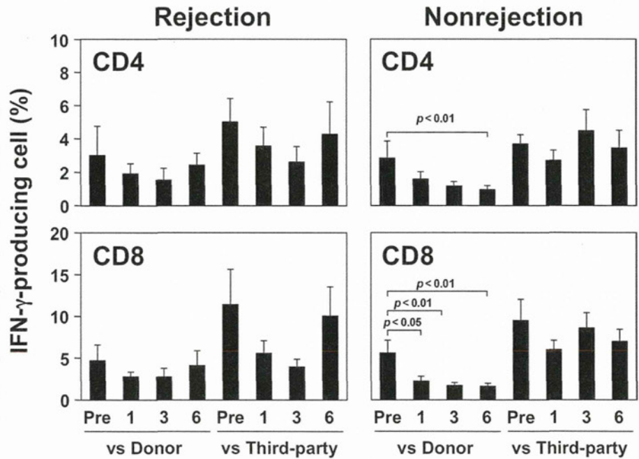
Fig 2. Temporal change in the frequencies of donor-specific T cells. PBMCs from the recipients were stimulated with CD40-activated B cells from the corresponding donors for 7 days, and each cell population was then restimulated for 5 hours with CD40-activated B cells from the donor or third party. After secondary stimulation, intracellular IFN- \gamma was analyzed flow cytometrically using FITC-anti-IFN- \gamma , PE-anti-CD69, and PC5-anti-CD4 or CD8. The average frequencies of IFN- \gamma -producing cells in the CD4 + CD69 + or CD8 + CD69 + cells at the indicated time points are shown. The bars represent the standard errors.
