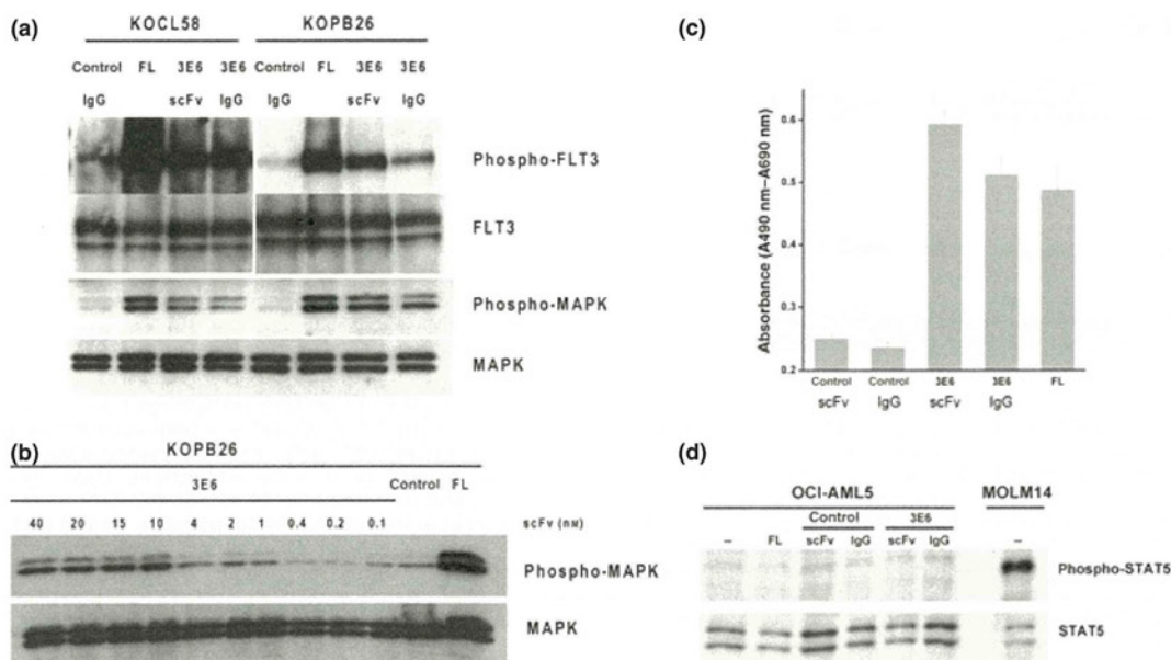
Fig. 2. Agonistic effects of 3E6 on KOCL58, KOPB26, and OCI-AML5 cells. (a) After the KOCL58 and KOPB26 cell lines were incubated with 3E6 IgG (67 nM), 3E6 scFv (200 nM) or the FMS-related tyrosine kinase 3 (FLT3) ligand (FL) (1.7 nM) for 10 min, FLT3 and MAPK phosphorylation were evaluated by immunoblotting. (b) After the KOPB26 cells were incubated with 3E6 scFv at concentrations ranging from 0.1 to 40 nM for 10 min, MAPK phosphorylation was examined by Western blotting. (c) Growth of the OCI-AML5 cells was examined with either FL alone (1.7 nM), 3E6 scFv (200 nM), 3E6 IgG (67 nM), or controls at 7 days' incubation. Cell growth was measured using the MTT assay. (d) Signal transducer and activator of transcription 5 (STAT5) phosphorylation on the OCI-AML5 cells with 3E6. MOLM14 cells, harboring the FLT3-ITD mutation, are the positive control.
