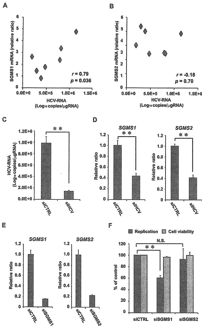
Figure 2. Relationship between the SGMS genes and HCV infection. (A, B) The correlation between SGMS1/2 and liver HCV-RNA of HCV infected humanized chimeric mice (n=7). (C) The effect of silencing HCV genome RNA with siRNA (siE-R7: 1 nM) on HCV in HCV-infected cells. (D) The effect of silencing HCV genome RNA with siRNA (siE-R7: 1 nM) on the expression of SGMS1/2 mRNA measured by RTD-PCR. (E) The effect of silencing SGMS1/2 mRNA with siRNA (3 nM each) measured by RTD-PCR. (F) The effect of silencing SGMS1/2 mRNA with siRNA (3 nM) on HCV replication in FLR 3-1. In all cases, error bars indicate SDs. * p <0.05 and ** p <0.01. doi:10.1371/journal.ppat.1002860.g002
