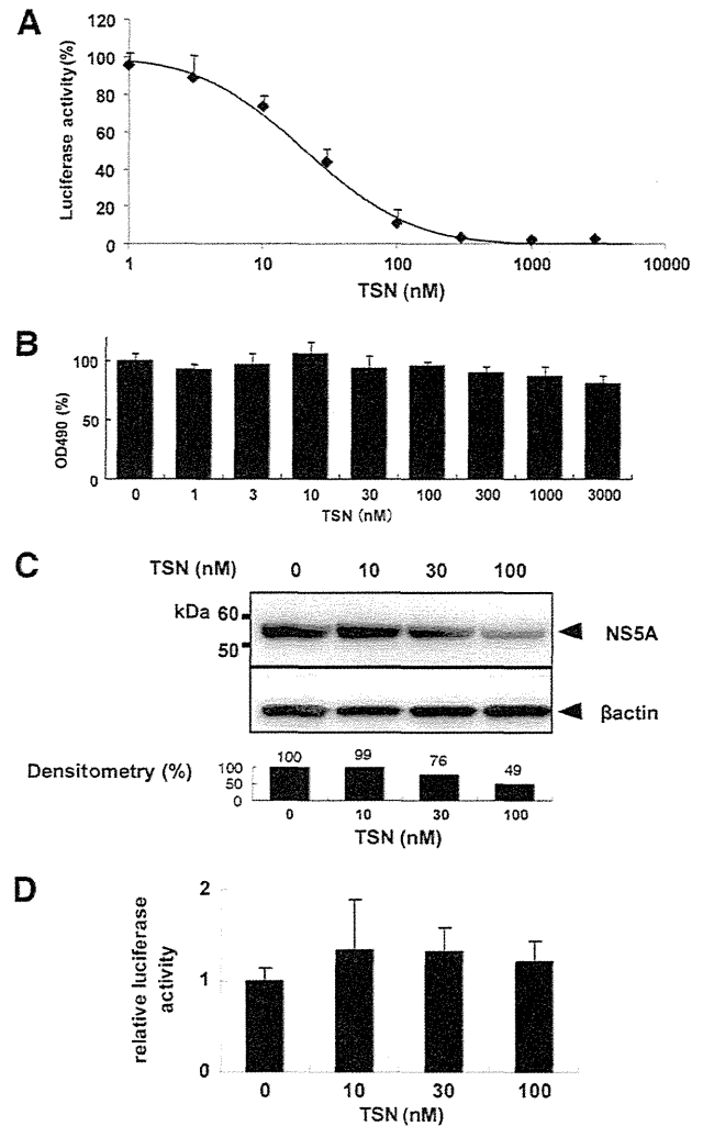
FIG. 2. Effect of TSN on expression of HCV replicon. (A) HCV replicon cells were treated with various concentrations of TSN for 48 h. Replication levels of HCV RNA were analyzed by luciferase assay. Bars indicate luciferase activities relative to that of the drug-negative control. (B) Cell viability was determined by MTS assay. Bars indicate the value relative to that of the drug-negative control. (C) Western blotting analyses. The expression of NS5A and beta-actin was detected using anti-NS5A and anti-beta-actin antibodies. Densitometry of NS5A protein was performed, and the result is indicated as a percentage of the result for the drug-negative control. The assay was repeated three times, and a representative result is shown. (D) A bicistronic reporter gene plasmid, pCIneo-Rluc-IRES-Fluc, was transfected into Huh7 cells. The cells were cultured with TSN at the concentrations indicated, and dual luciferase activities were measured after 24 h of treatment. Values are displayed as ratios of Fluc to Rluc. In panels A, B, and D, the assays were done in triplicate and repeated three times. Error bars indicate means \pm SDs.
