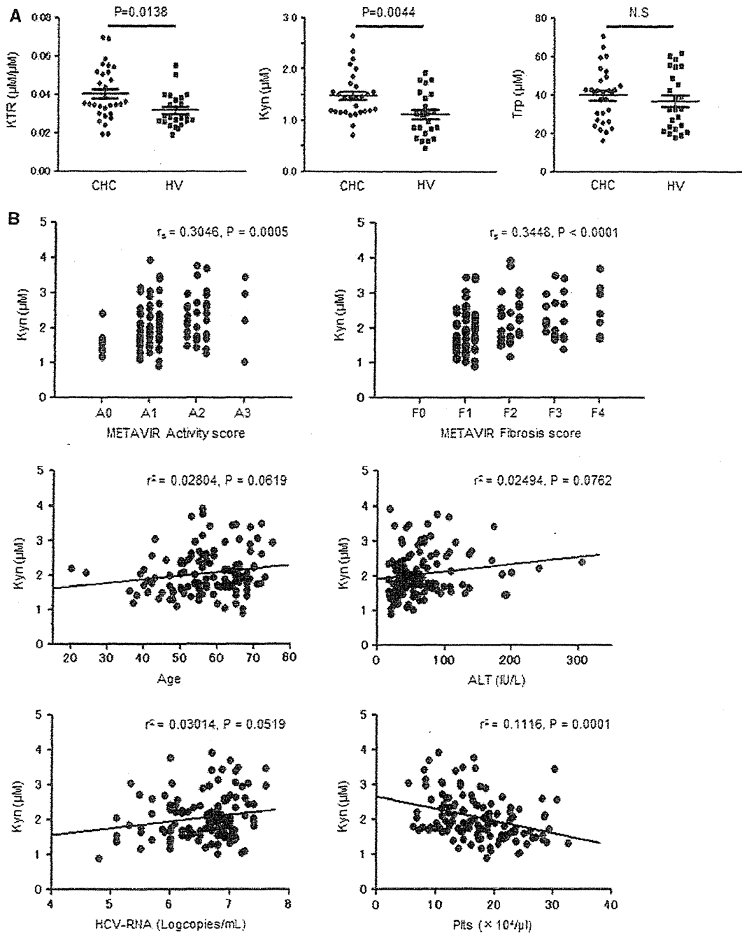
Fig. 1 Systemic indoleamine 2,3-dioxygenase (IDO) activity is enhanced in chronic hepatitis C patients. a Serum kynurenine (Kyn) and tryptophan (Trp) were assayed by HPLC as described in “Subjects, materials, and methods”, and the kynurenine-to-tryptophan ratio (KTR) was calculated from their concentrations. Scatter plots of 30 chronic hepatitis C patients (CHC) and 24 healthy volunteers (HV) are shown. Horizontal bars depict mean \pm SEM. Statistical analyses were performed using the nonparametric Mann-
