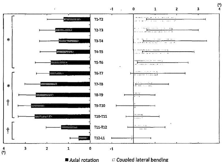
Figure 3. Mean range of motions (bar) and SD (line) of axial rotations (left) and coupled lateral bending (right) of 1 side during trunk rotations. * P < 0.01 .
