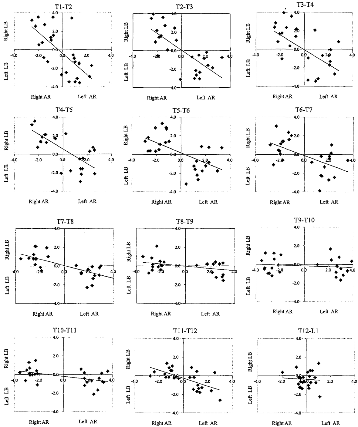
Figure 4. Relationships between axial rotation (AR) and coupled lateral bending (LB) at each spinal segment. The degree of AR was plotted on the x axis and the degree of coupled LB was plotted on the y axis. A negative slope of approximate curve meant coupled LB occurred in the same direction as AR.
