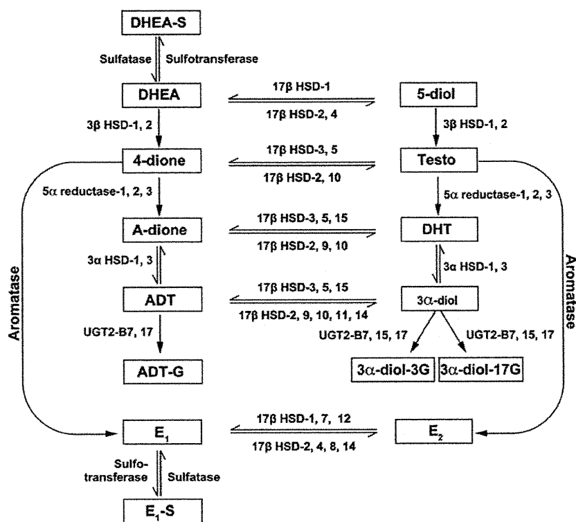
FIG. 1. Measured steroids and their metabolic relationships. 5-diol, Androst-5-ene-3 \beta ,17 \beta -diol; A-dione, androstenedione; E2, estradiol; E1, estrone; E1-S, estrone sulfate; HSD, hydroxysteroid dehydrogenase. [Adapted from Refs. 41–43.]
