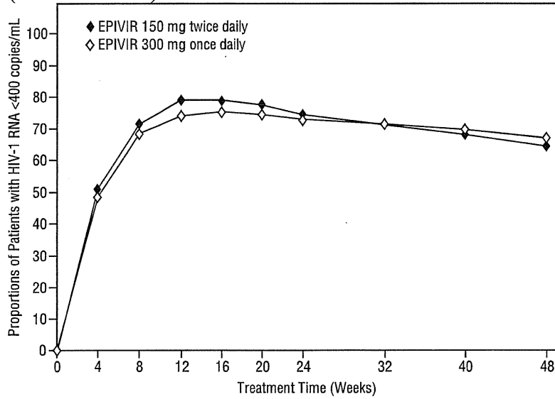
Figure 1. Virologic Response Through Week 48, EPV20001*† (Intent-to-Treat)
