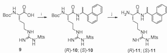
Scheme 2. Synthetic schemes of Unit 2, compounds ( R/S )- 11 . Reagents and conditions: (i) EDCl-HCl, \text{HOBT}\cdot\text{H}_2\text{O} , \text{Et}_3\text{N} , ( R/S )-(+/-)-1-(1-naphthyl)ethylamine, \text{CH}_2\text{Cl}_2 , 83–97%; (j) TFA then 4 M \text{HCl}/\text{EtOAc} , quantitative; EDCl-HCl = 1-ethyl-3-(3-dimethylaminopropyl)carbodiimide hydrochloride, \text{HOBT}\cdot\text{H}_2\text{O} = 1-hydroxybenzotriazol monohydrate, Mts = 2,4,6-trimethylphenylsulfonyl, Boc = tert -butoxycarbonyl.
