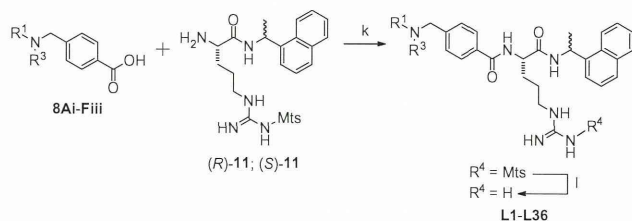
Scheme 3. Synthetic schemes of compounds 12–47 . Reagents and conditions: (k) EDCl-HCl, \text{HOBT}\cdot\text{H}_2\text{O} , \text{Et}_3\text{N} , \text{DMF} , 36–95%; (l) TMSBr, m -cresol, 1,2-ethanedithiol, thioanisole, TFA, 4–54%. The structures of \text{R}^1 and \text{R}^3 are shown in Figure 2 as i–iii and A–F, respectively.
