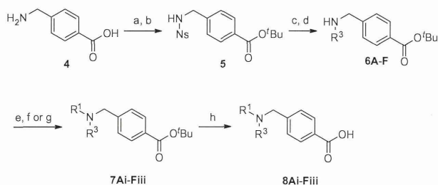
Scheme 1. The synthetic scheme of Unit 1, compounds 8Ai-Fiii . Reagents and conditions and yields: (a) \text{NscI} , \text{Et}_3\text{N} , \text{THF}/\text{H}_2\text{O} (1/1); (b) isobutene, \text{THF}/\text{H}_2\text{SO}_4 (10/1), 39% (2 steps); (c) \text{PPh}_3 , \text{DEAD} , \text{R}^2\text{OH} , \text{THF} ; (d) \text{PhSH} , \text{K}_2\text{CO}_3 , \text{DMF} , 42–92% (2 steps); (e) \text{NaBH}(\text{OAc})_3 , 4-fluorobenzaldehyde, \text{CH}_2\text{Cl}_2 ; (f) \text{NaBH}(\text{OAc})_3 , (4-fluorophenyl)acetaldehyde, \text{CH}_2\text{Cl}_2 ; (g) 4-fluorobenzoyl chloride, \text{Et}_3\text{N} , \text{CH}_2\text{Cl}_2 , 51–94%; (h) TFA then 4 M \text{HCl}/\text{EtOAc} , quantitative; The structures of \text{R}^1 and \text{R}^3 are shown in Fig. 2 as i–iii and A–F, respectively. \text{Ns} = 2-nitrobenzenesulfonyl, \text{tBu} = tert -butyl, \text{DEAD} = diethyl azodicarboxylate.
