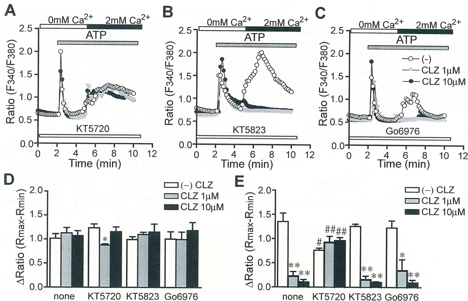
Supplemental Figure VII. PKA-dependent suppression of TRPC6-mediated \text{Ca}^{2+} influx by PDE3 inhibition. (A-C) Average time courses of \text{Ca}^{2+} responses induced by ATP in TRPC6-expressing cells in the presence of PKA inhibitor (KT5720) (A), PKG inhibitor (KT5823) (B), and PKC inhibitor (Go6976) (C). Cells were pretreated with indicated concentration of cilostazol (CLZ) with KT5823 (0.3 \mu\text{M} ), KT5720 (0.1 \mu\text{M} ), or Go6976 (20 nM) for 30 min before stimulation with ATP (100 \mu\text{M} ). (D, E) Peak \text{Ca}^{2+} release-mediated [\text{Ca}^{2+}]_i increases (D) and \text{Ca}^{2+} influx-mediated [\text{Ca}^{2+}]_i increases (E) induced by ATP in the absence or presence of CLZ. *, P < 0.05 , **, P < 0.01 vs CLZ (-), #, P < 0.05 , ###, P < 0.01 vs none.
