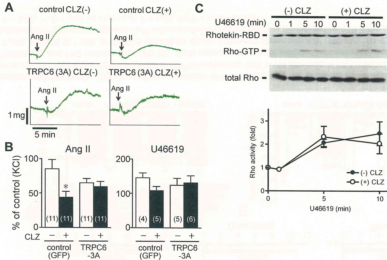
Supplemental Figure VIII. Inhibition of TRPC6 abolishes suppression of Ang II-induced contraction by PDE3 inhibition. (A) Representative time courses of changes in aortic ring tensions reconstituted from primary cultured RAOsMC expressing GFP or dominant negative mutant of TRPC6 (TRPC6-3A). CLZ (10 \mu M) was treated for 30 min before stimulation with Ang II (100 nM). (B) Peak contraction induced by Ang II and U46619 in the absence (-) or presence (+) of CLZ in control (GFP)- and TRPC6-3A-expressing RAOsMC. *, P < 0.05 vs control CLZ(-). (C) Effects of CLZ on agonist-induced Rho activation. RAOsMC were pretreated with CLZ for 30 min before stimulation of thromboxane A2 receptor with U46619 (100 nM). N=3 experiments.
