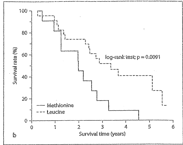
Fig. 1. Cumulative survival rates according to substitution of core amino acid in the elderly group. a Cumulative survival rate according to Gln70/His70 was not different compared with that related to Arg70. b Cumulative survival rate in Met91 was significantly lower than in Leu91.
