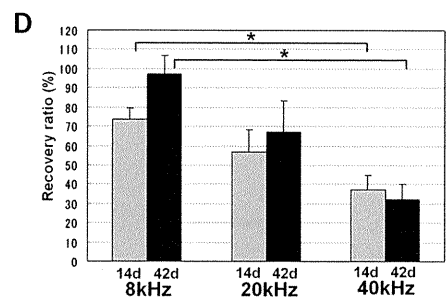
Figure 1. ABR threshold shift and hearing recovery ratio after 3NP administration to the inner ear. A–C: ABR thresholds of 8 ( A ), 20 ( B ), and 40 kHz ( C ) were monitored for 6 weeks. Solid circles , 3NP-treated rats; open triangles , saline controls. D: Hearing recovery ratios (peak threshold – threshold at 14 days or 42 days/peak threshold \times 100) were calculated from ABR thresholds. At 14 and 42 days, the recovery ratio of ABR threshold for 8 kHz were significantly higher ( P = 0.0005 and 0.005 , respectively) than the ratio for 40 kHz. Asterisk indicates statistical significance ( P < 0.05 ).
