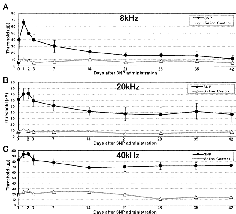
Figure 1. ABR threshold shift and hearing recovery ratio after 3NP administration to the inner ear. A–C: ABR thresholds of 8 ( A ), 20 ( B ), and 40 kHz ( C ) were monitored for 6 weeks. Solid circles , 3NP-treated rats; open triangles , saline controls. D: Hearing recovery ratios (peak threshold – threshold at 14 days or 42 days/peak threshold \times 100) were calculated from ABR thresholds. At 14 and 42 days, the recovery ratio of ABR threshold for 8 kHz were significantly higher ( P = 0.0005 and 0.005 , respectively) than the ratio for 40 kHz. Asterisk indicates statistical significance ( P < 0.05 ).
