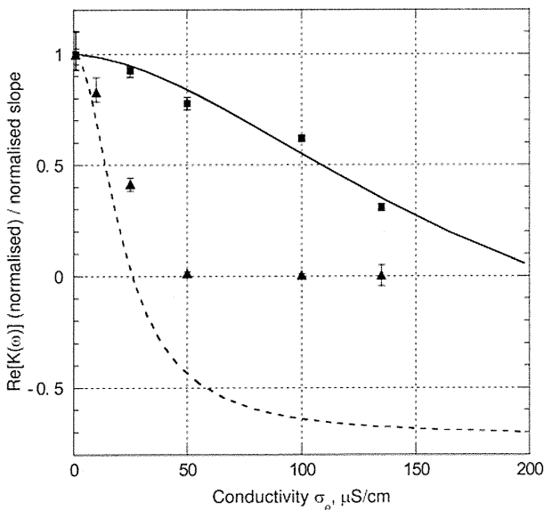
Fig. 5 Theoretical calculations of \text{Re}[K(\omega)] (solid, 800 kHz; dashed, 100 kHz) and experimental results of DEPIM at E. coli concentration of 5 \times 10^5 \text{ CFU/ml} ( \blacksquare , 800 kHz; \blacktriangle , 100 kHz), these were normalised to these values at low medium conductivity ( 1 \mu\text{S cm}^{-1} )
