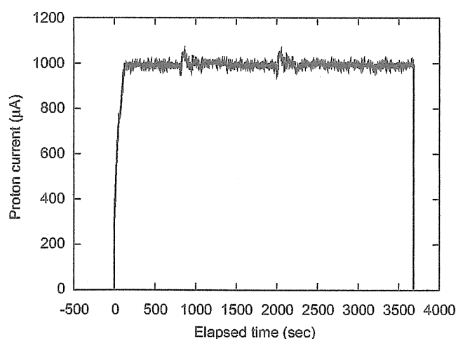
Fig. 2. Relationship between elapsed time and proton current detected at the beryllium target.
