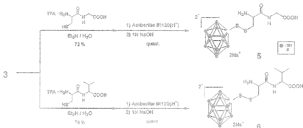
Fig. 5. Synthesis of Thiododecaborate-Containing Dipeptides.
