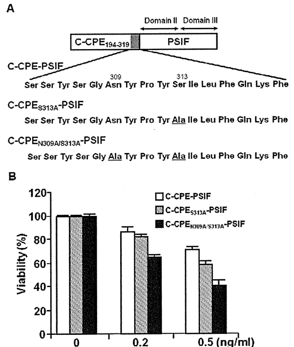
Figure 1. Cytotoxicity of C-CPE-PSIF fusion proteins (A) Schematic illustration of C-CPE-PSIF fusion proteins. C-CPE is the C-terminal fragment of CPE corresponding to amino acids 194-319. The dark area indicates the putative claudin-4-binding region (15). Changing Asn to Ala at position of 309 or Ser to Ala at position of 313 improved the affinity of C-CPE to claudin-4 (14). C-CPE S313A or C-CPE N309A/S313A -fused PSIF was also prepared. PSIF contains domain II (the critical domain for the escape of the toxin from the endosome to the cytosol) and domain III (the critical domain for the inhibition of protein synthesis) of Pseudomonas exotoxin. (B) Cytotoxicity of C-CPE-PSIF. CL4/L cells were treated with the C-CPE-PSIF fusion proteins at the indicated concentration for 24 h. The cellular viability was measured by a WST-8 assay kit, according to the manufacturer's instructions (Nacalai Tesque, Kyoto, Japan). Viability (%) was calculated as a percentage of the vehicle-treated cells. The data represent the mean \pm SD of three independent experiments.
