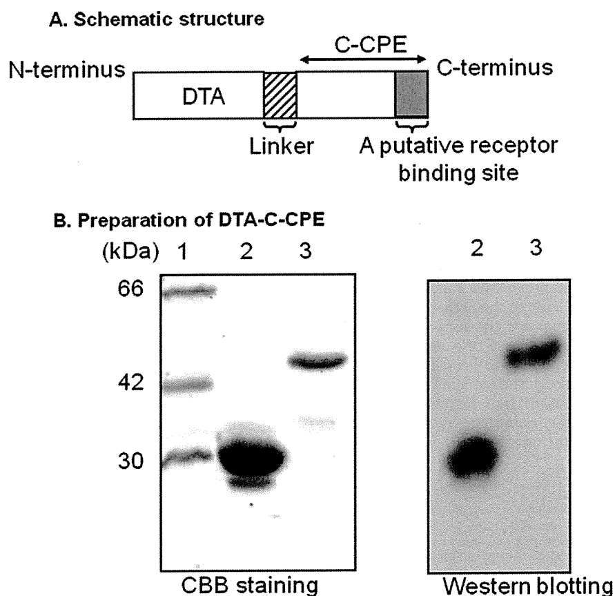
Fig. 1. Preparation of DTA-C-CPE. (A) Schematic structure of DTA-C-CPE. DTA-C-CPE is a fusion protein of DTA and C-CPE with a linker indicated by a slashed column. A dark column indicates a putative receptor-binding region of C-CPE. (B) Preparation of DTA-C-CPE. DTA or DTA-C-CPE was produced by a conventional expression system of E. coli , and the proteins were purified by His-tag affinity chromatography with Ni-resins. The purification of DTA-C-CPE was confirmed by SDS-PAGE followed by staining with Coomassie Brilliant Blue (CBB) (left panel in B) and by Western blotting using an anti-His-tag mAb (right panel in B). Lane 1, a marker of molecular size; lane 2, DTA; lane 3, DTA-C-CPE. The putative molecular sizes of DTA and DTA-C-CPE were 30 and 43.2 kDa, respectively.
