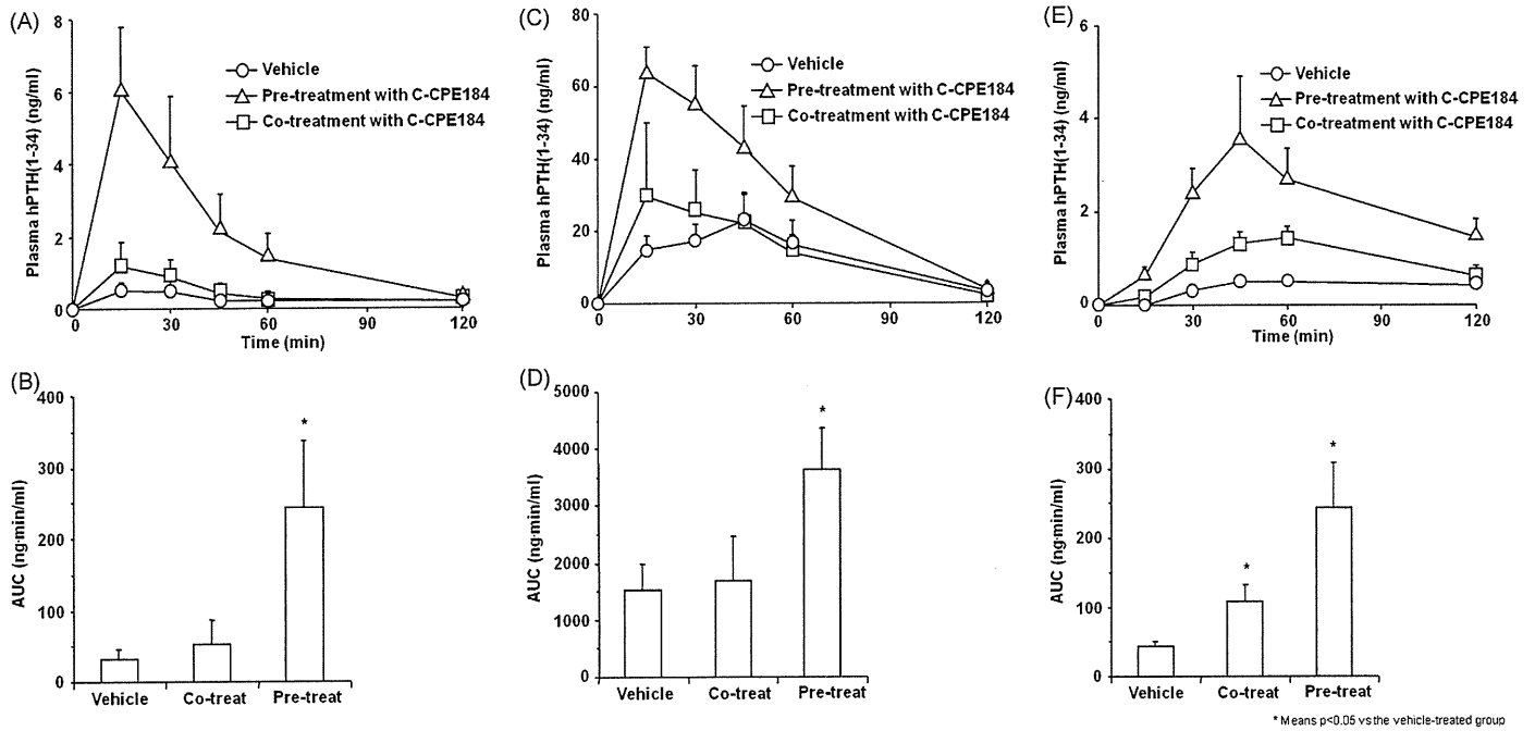
Fig. 1. Effect of C-CPE184 on mucosal absorption of hPTH(1-34) in rats. (A, B) Jejunal absorption of hPTH(1-34). Jejunum was co-treated with hPTH(1-34) (100 µg) and C-CPE184 (20 µg), or jejunum was treated with hPTH(1-34) 4 h after treatment with C-CPE184. (C, D) Pulmonary absorption of hPTH(1-34). hPTH(1-34) (150 µg) was pulmonary administered with C-CPE184 (5 µg) or 4 h after administration of C-CPE184. (E, F) Nasal absorption of hPTH(1-34). hPTH(1-34) (200 µg) was nasally administered with C-CPE184 (2 µg) or 4 h after administration of C-CPE184. Plasma hPTH(1-34) levels were measured at the indicated periods. Time-course changes in plasma hPTH(1-34) levels (A, C, E) and AUC from 0 to 120 min (B, D, F) were calculated. Data are mean ± SE (n = 3–6). Co-treat indicates co-treatment with both hPTH and C-CPE184, and Pre-treat indicates treatment with hPTH 4 h after C-CPE184-treatment. *Significantly different from the vehicle-treated group (p < 0.05).
