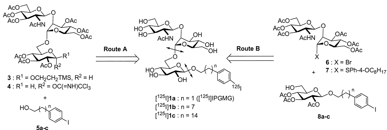
Scheme 1. Retrosynthetic strategy of [^{125}\text{I}] radiolabeled trisaccharide derivatives ( [^{125}\text{I}]1\mathbf{a-c} )
