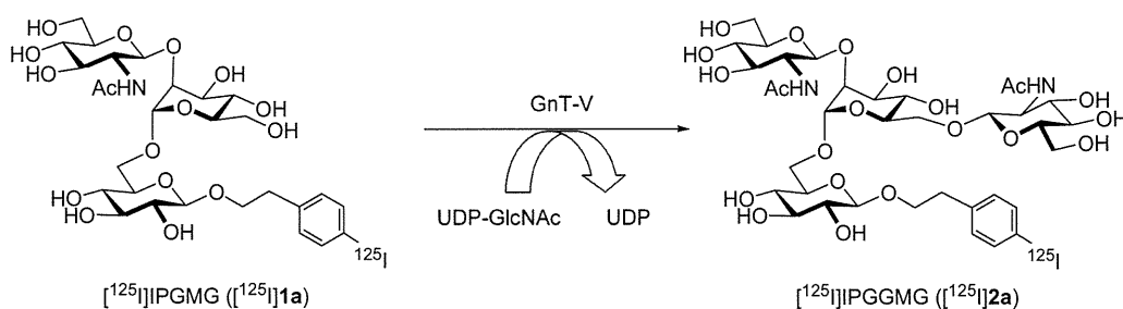
Figure 1. The transfer of a GlcNAc residue from UDP-GlcNAc to [^{125}\text{I}]1 to form [^{125}\text{I}]2 by GnT-V
