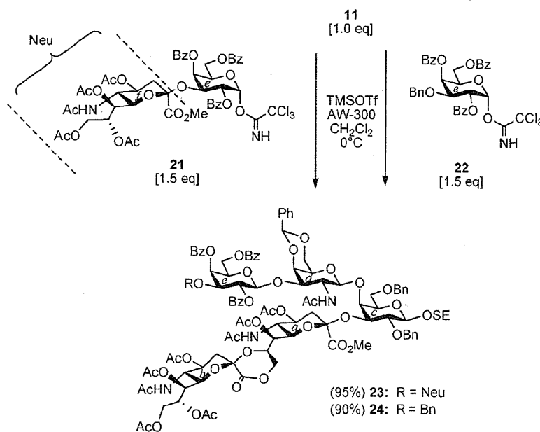
SCHEME 4. Potential as an Acceptor of 11 for the Systematical Synthesis of B-Series Gangliosides
