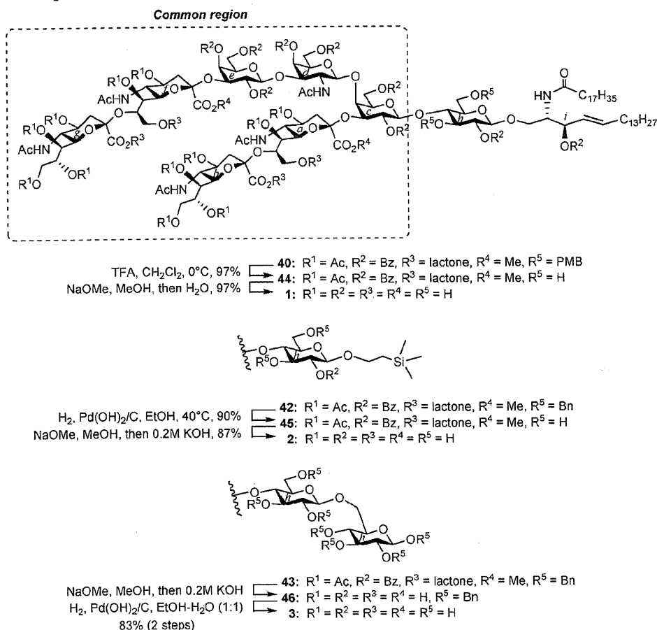
SCHEME 6. Global Deprotections
