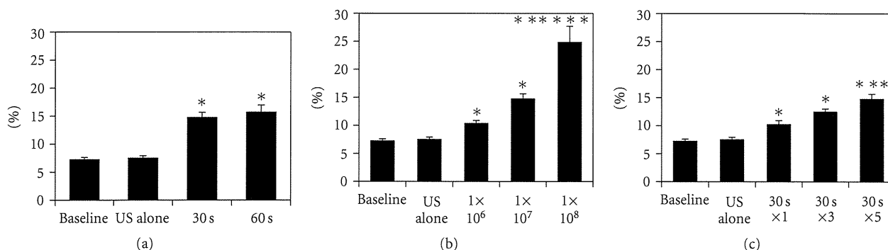
FIGURE 4: (a) Effect of insonification time on cell viability using 60 µg of DNA, 1 × 10 7 particles/mL liposome, and 15-min incubation with DNA, and three 30- or 60-sec insonifications. “US alone” represents the percentage of dead cells immediately after three 30-sec insonifications in the absence of liposome and DNA. * P < .05 versus baseline. (b) Effect of liposome concentration on cell viability using 60 µg of DNA and three 30-sec insonifications and 15-min incubation with DNA. * P < .05 versus baseline; ** P < .05 versus 1 × 10 6 particles/mL; *** P < .05 versus 1 × 10 8 particles/mL. (c) Effect of repetitions of insonification on cell viability using 60 µg of DNA, 1 × 10 7 particles/mL liposome, and 15-min incubation with DNA. * P < .05 versus baseline; ** P < .05 versus 30 sec × 1.
