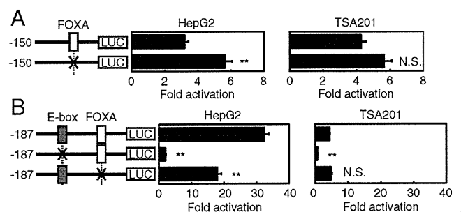
FIG. 2. Changes in hDIO1 promoter activity by FOXA binding site and E-box. Schematic diagram in the left of each figure representing WT and site-specific mutations of the hDIO1 promoter, introduced into the upstream region of the luciferase gene. A cross represents the site-specific mutation of the putative FOXA binding site or E-box. Each construct was transiently transfected into HepG2 or TSA 201 cells. Promoter activity was normalized to Renilla luciferase activity and expressed as the relative activity to promoterless pGL4.10. Statistical significance was determined by unpaired t test (A) or ANOVA followed by Dunnett's test (B). **, P < 0.01 . N.S., Not significant.
