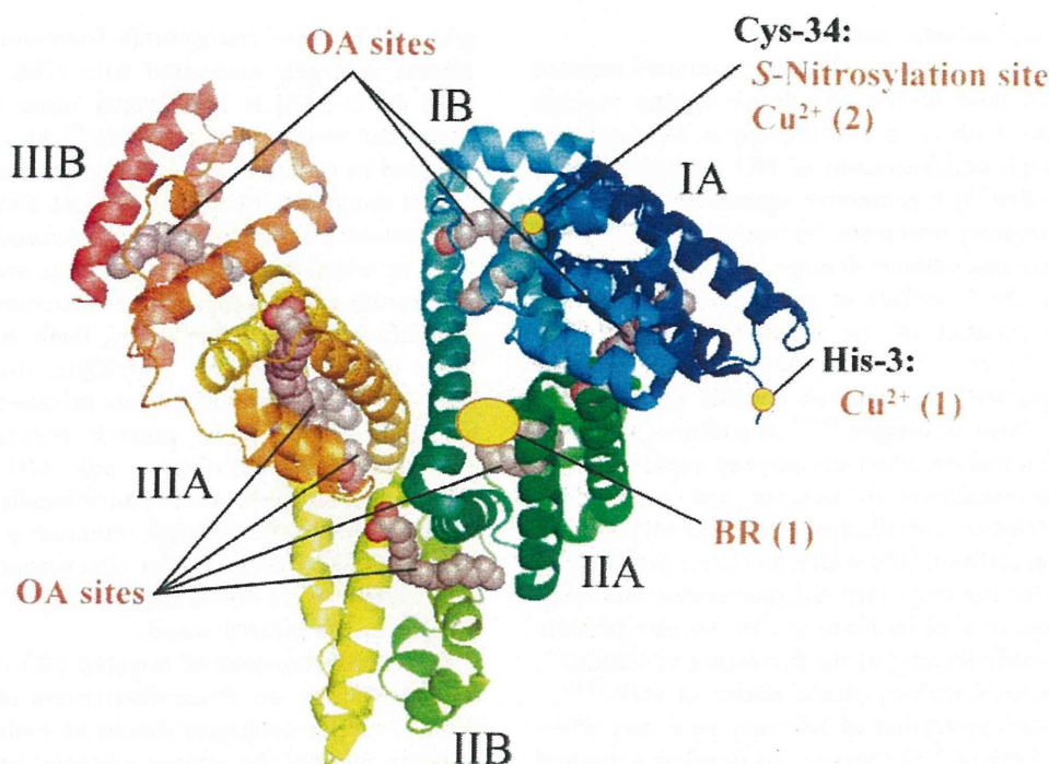
Fig. 1. Crystal structure of HSA showing locations of Cys-34 and OA, BR and \text{Cu}^{2+} binding sites
