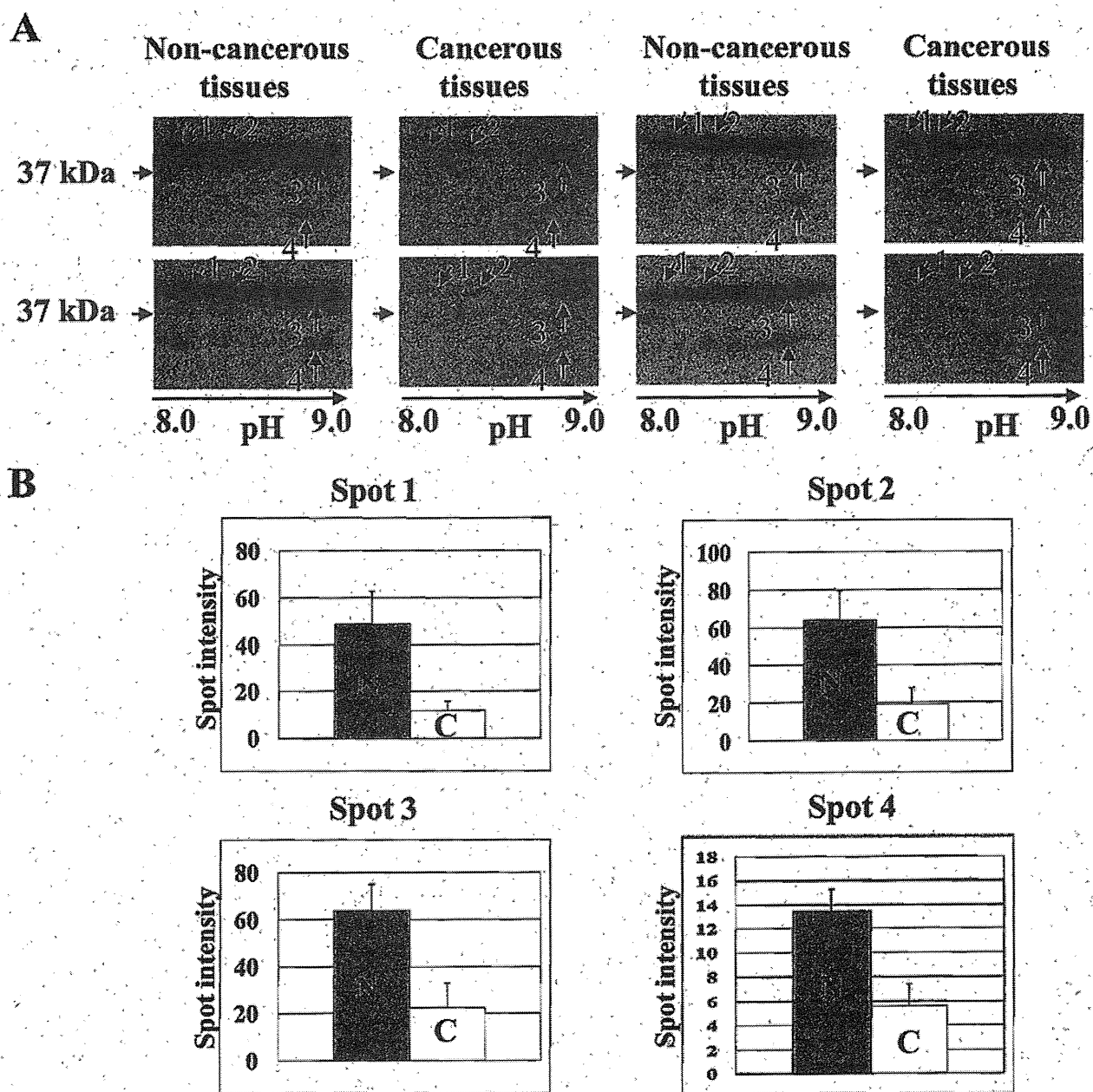
Figure 3. 2-D Western blot analysis of aldolase B. A: Four pairs of cancerous and paired non-cancerous tissues from patients with HCV-HCC underwent 2-D Western blot analysis. Using specific anti-aldolase B antibody, the spots were confirmed as four aldolase B isoforms. Each spot number is the same as those shown in Figure 1A. B: The differential intensities of protein spots in non-cancerous tissues (N) and cancerous tissues (C) in HCC were quantified by Student's t -test ( n=4 , p<0.05 for each spot). The error bars represent standard errors of the means.
